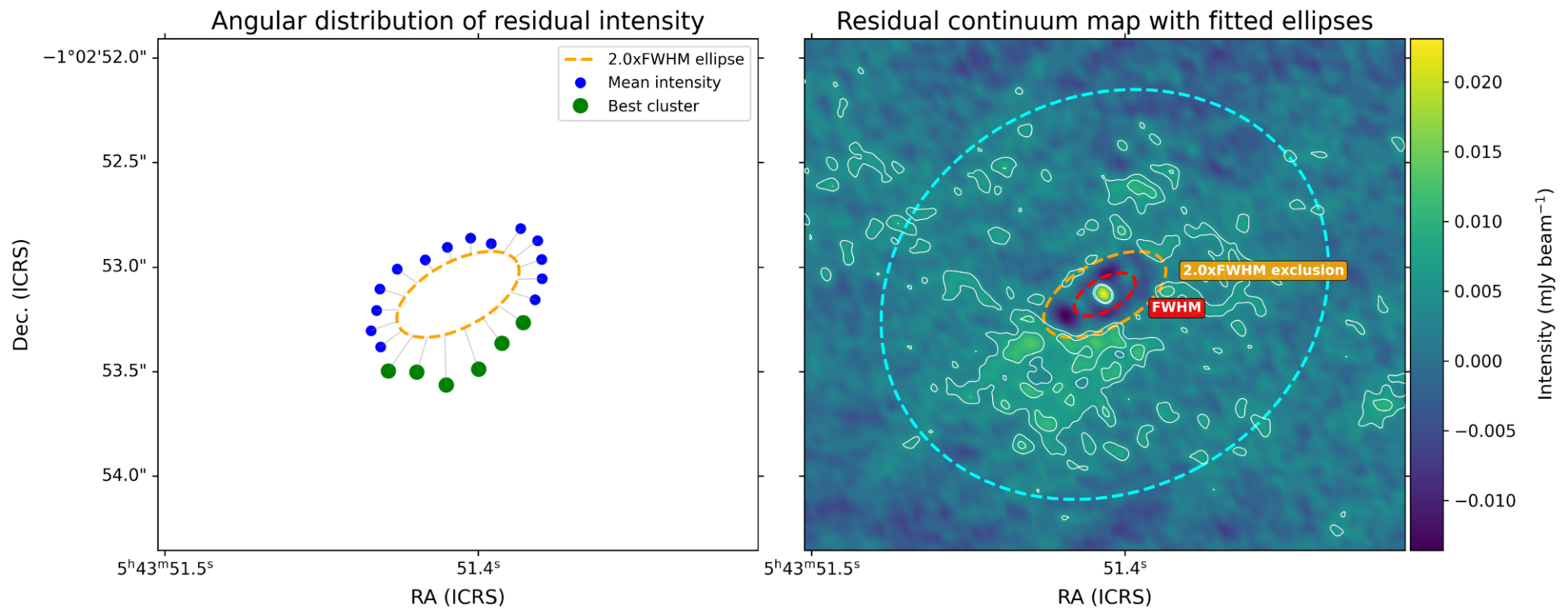
Figure D1. from Adele L. Plunkett et al 2026 Astron. J. 172 doi:10.3847/1538-3881/aeacc2 https://dx.doi.org/10.3847/1538-3881/aeacc2 © 2026. The Author(s). Published by the American Astronomical Society.
