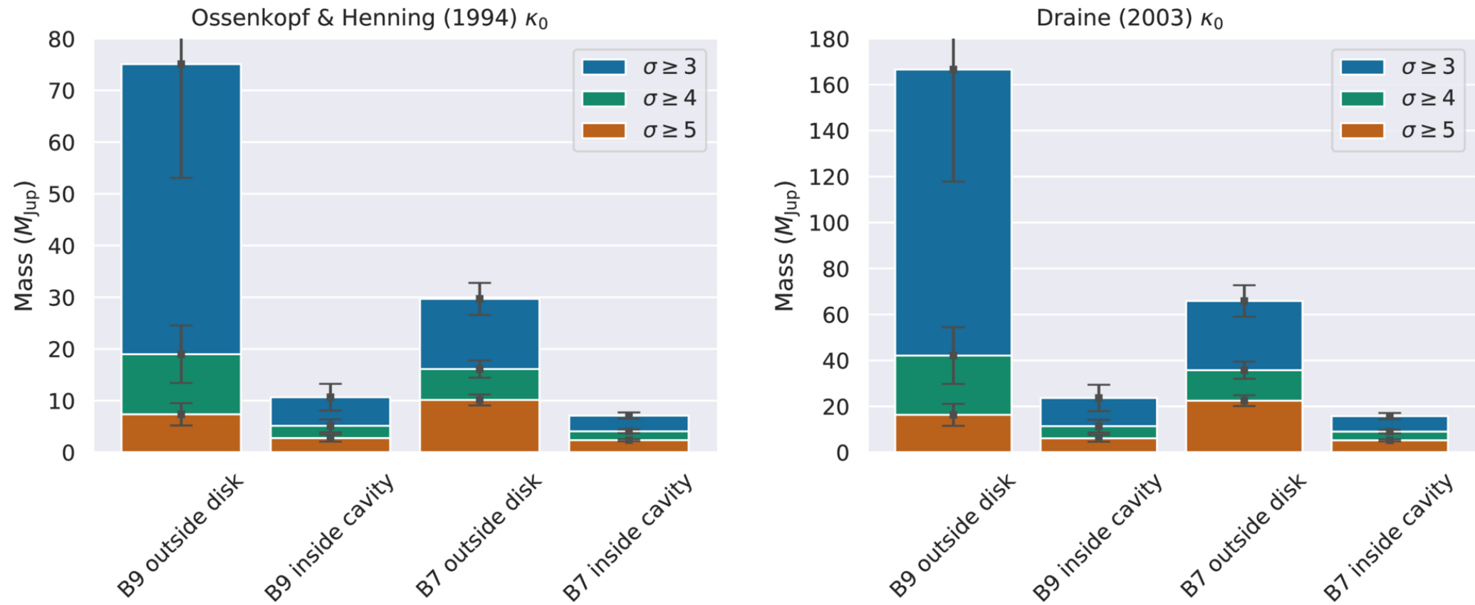
Figure 6. from Adele L. Plunkett et al 2026 Astron. J. 172 doi:10.3847/1538-3881/aeacc2 https://dx.doi.org/10.3847/1538-3881/aeacc2 © 2026. The Author(s). Published by the American Astronomical Society.
