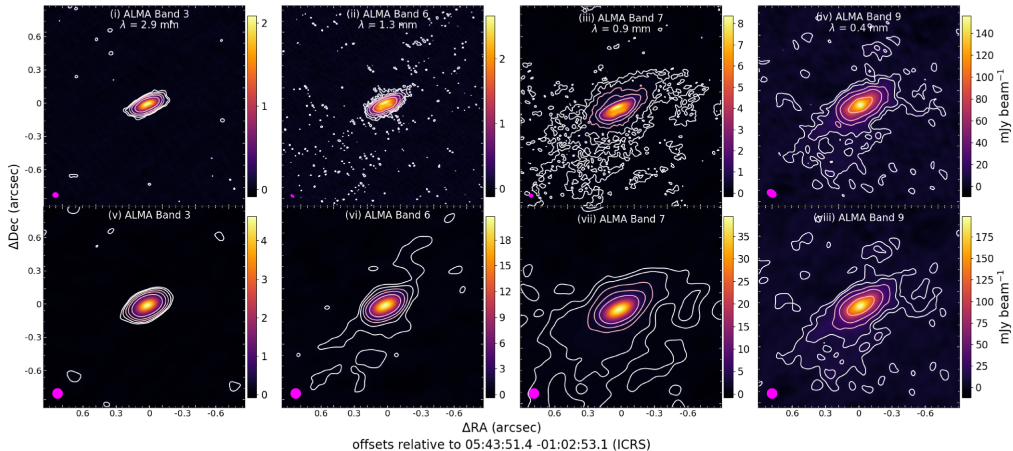
Figure 2. from Adele L. Plunkett et al 2026 Astron. J. 172 doi:10.3847/1538-3881/aeacc2 https://dx.doi.org/10.3847/1538-3881/aeacc2 © 2026. The Author(s). Published by the American Astronomical Society.
