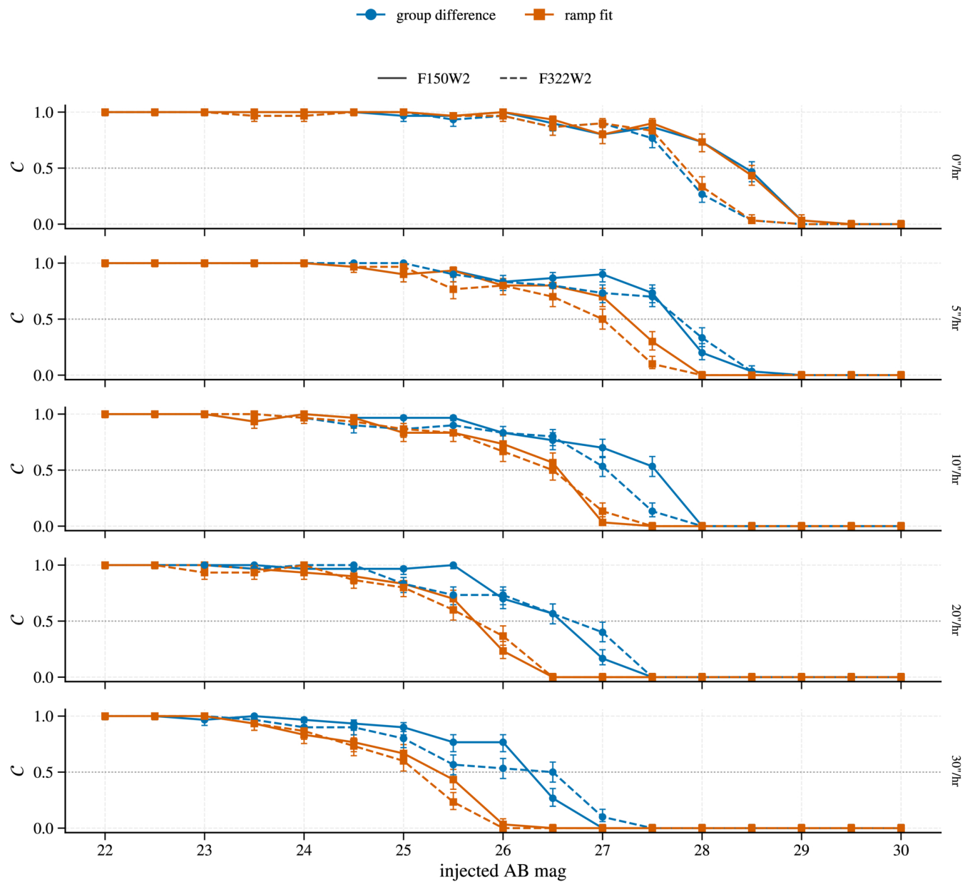
Figure 9. from Anthony Girmenia and Stanimir Metchev 2026 Astron. J. 172 doi:10.3847/1538-3881/aeab8a https://dx.doi.org/10.3847/1538-3881/aeab8a © 2026. The Author(s). Published by the American Astronomical Society.
