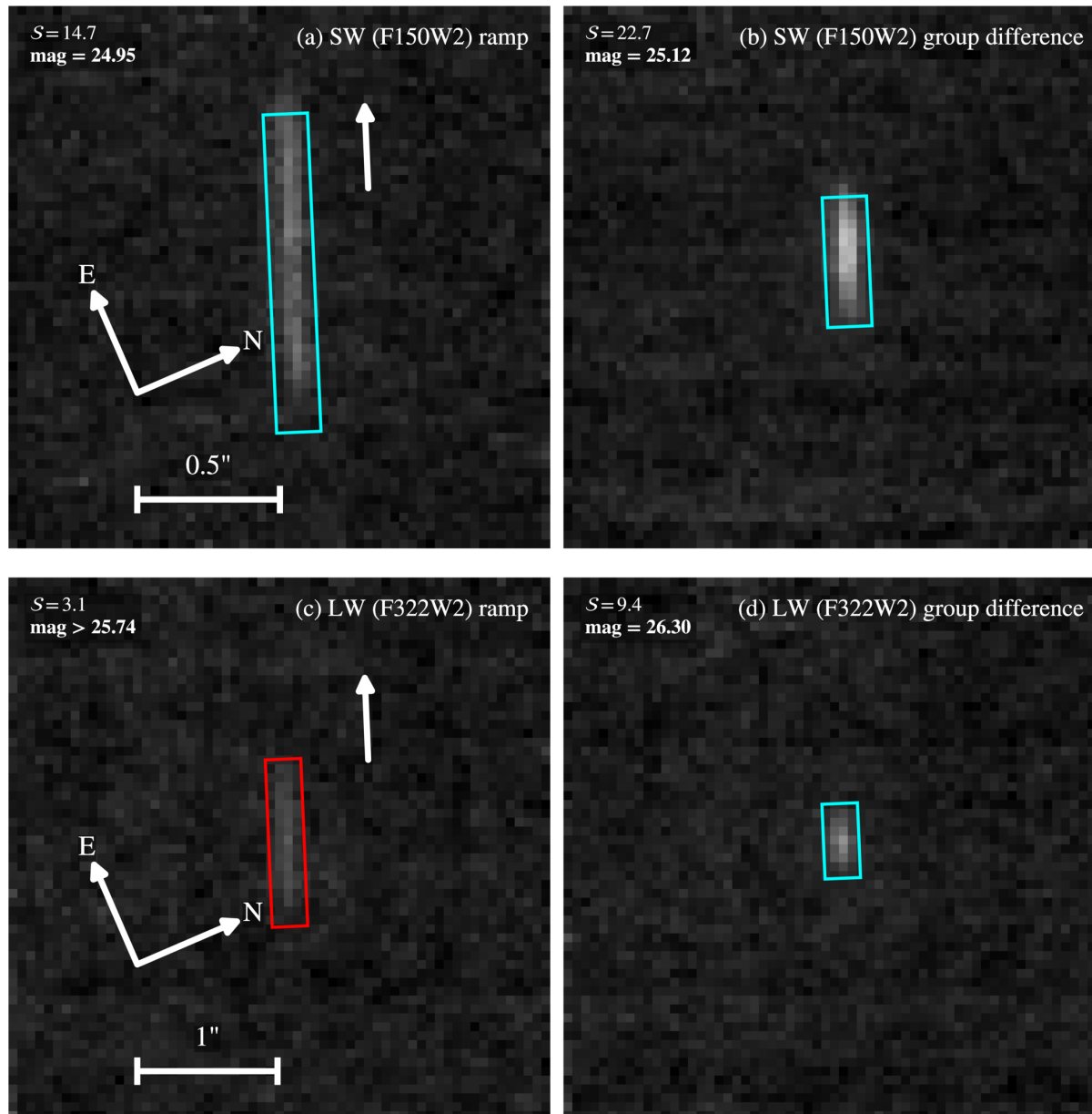
Figure 5. from Anthony Girmenia and Stanimir Metchev 2026 Astron. J. 172 doi:10.3847/1538-3881/aeab8a https://dx.doi.org/10.3847/1538-3881/aeab8a © 2026. The Author(s). Published by the American Astronomical Society.
