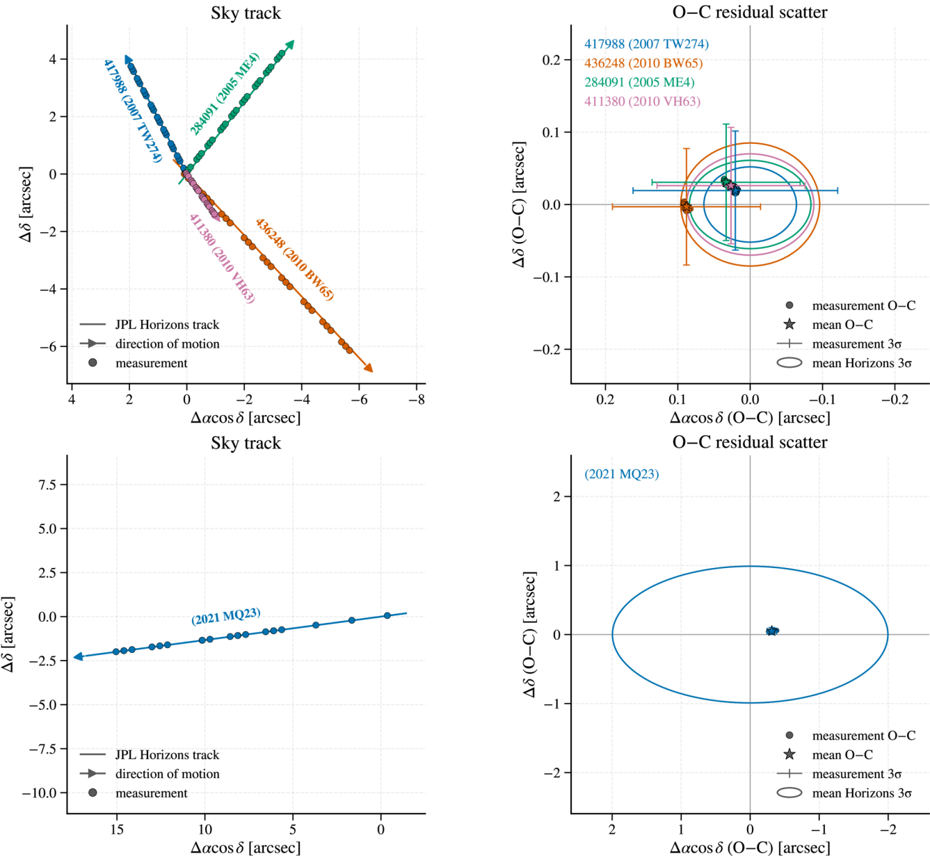
Figure 4. from Anthony Girmenia and Stanimir Metchev 2026 Astron. J. 172 doi:10.3847/1538-3881/aeab8a https://dx.doi.org/10.3847/1538-3881/aeab8a © 2026. The Author(s). Published by the American Astronomical Society.
