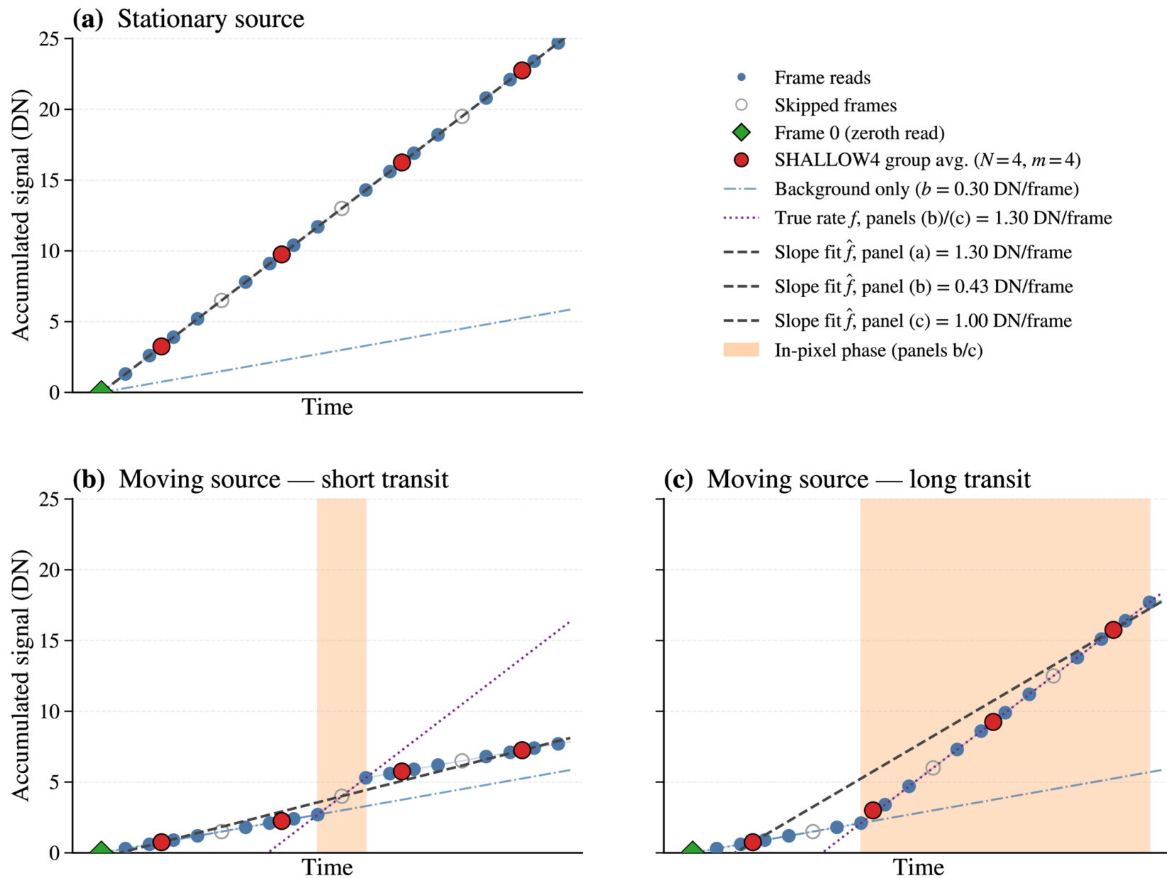
Figure 1. from Anthony Girmenia and Stanimir Metchev 2026 Astron. J. 172 doi:10.3847/1538-3881/aeab8a https://dx.doi.org/10.3847/1538-3881/aeab8a © 2026. The Author(s). Published by the American Astronomical Society.
