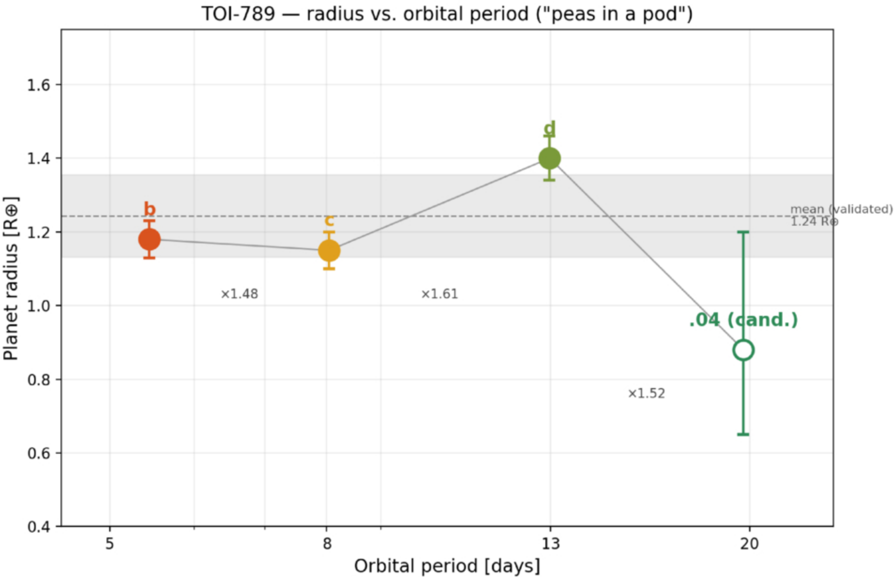
Figure 9. from Juan F. Pagés Navarrete 2026 Astron. J. 172 doi:10.3847/1538-3881/aea6c9 https://dx.doi.org/10.3847/1538-3881/aea6c9 © 2026. The Author(s). Published by the American Astronomical Society.
