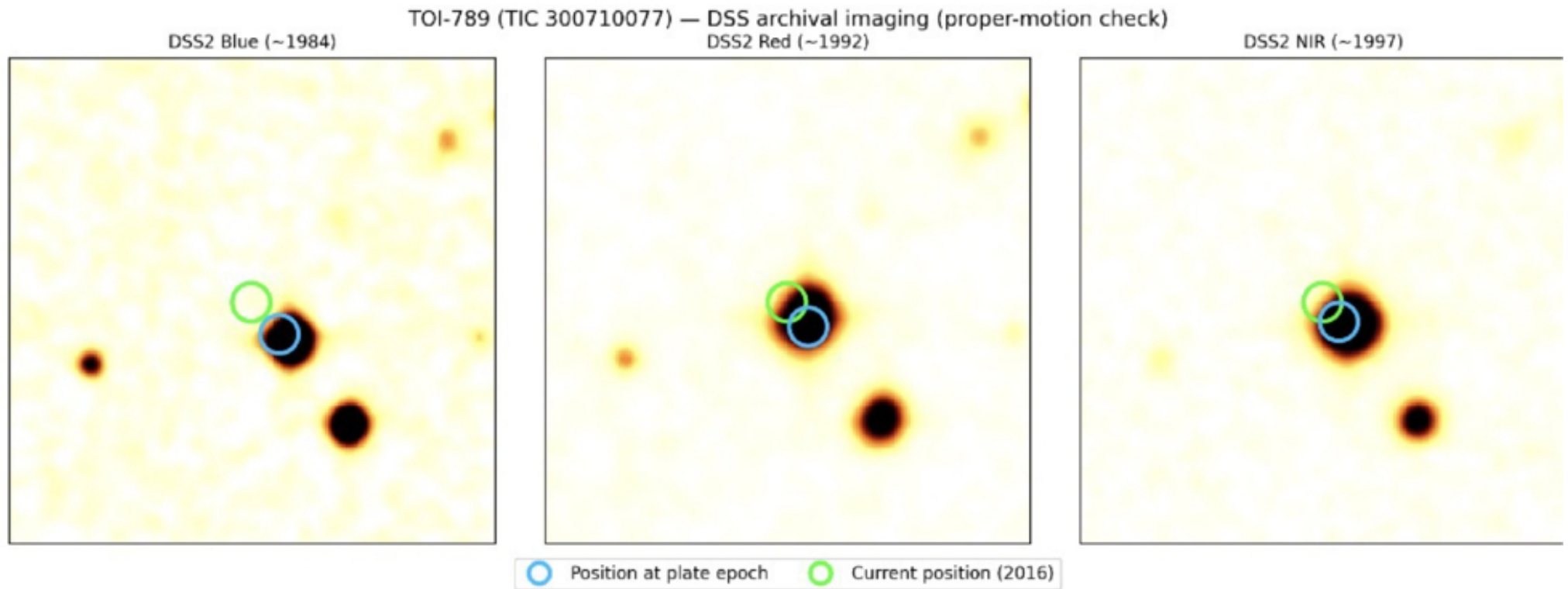
Figure 5. from Juan F. Pagés Navarrete 2026 Astron. J. 172 doi:10.3847/1538-3881/aea6c9 https://dx.doi.org/10.3847/1538-3881/aea6c9 © 2026. The Author(s). Published by the American Astronomical Society.
