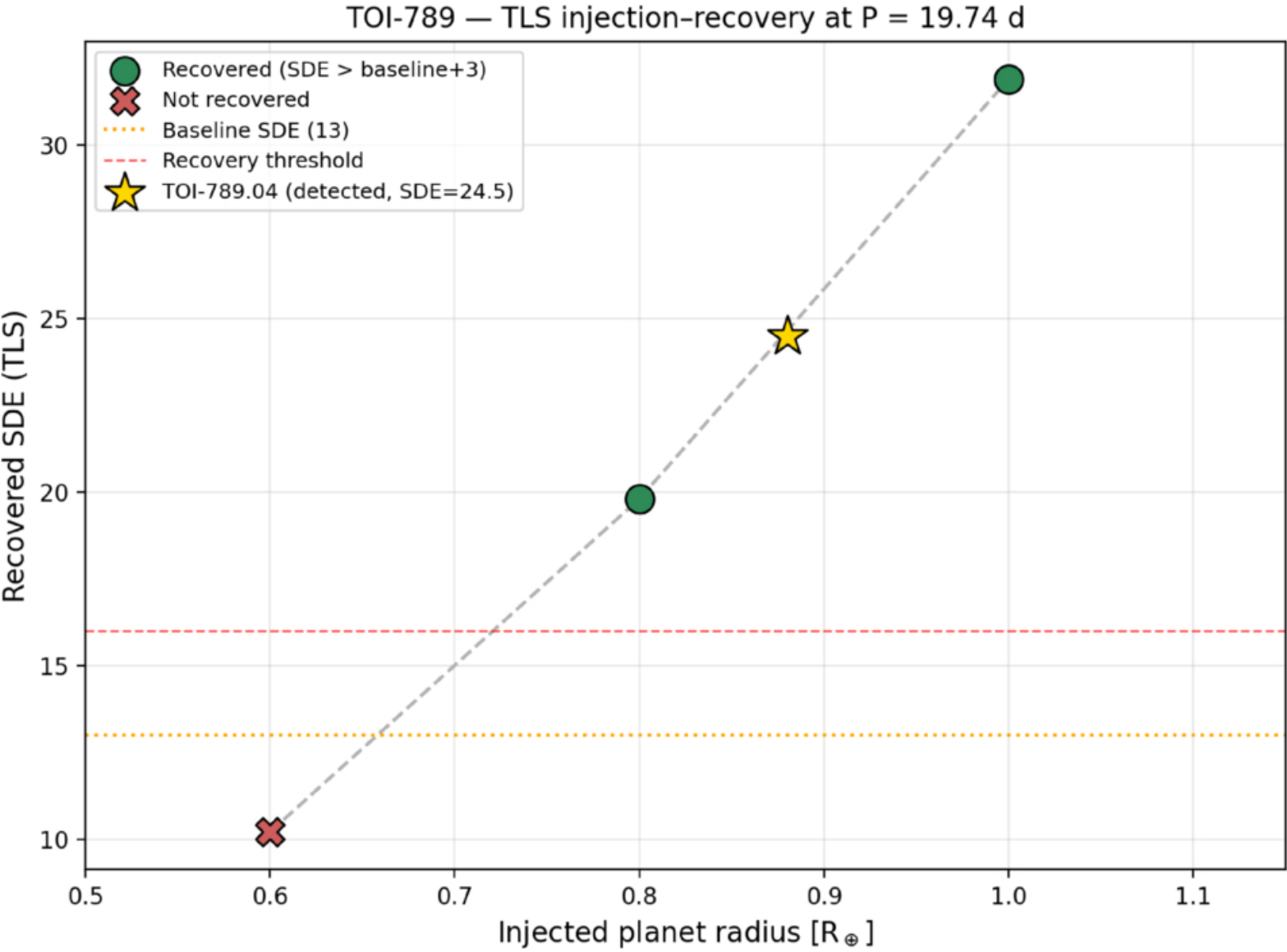
Figure 4. from Juan F. Pagés Navarrete 2026 Astron. J. 172 doi:10.3847/1538-3881/aea6c9 https://dx.doi.org/10.3847/1538-3881/aea6c9 © 2026. The Author(s). Published by the American Astronomical Society.
