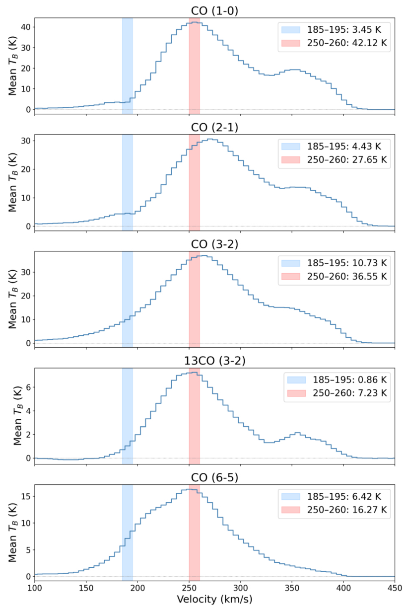
Figure 9. from Kaitlyn E. Sheriff et al 2026 Astron. J. 172 doi:10.3847/1538-3881/aea6ac https://dx.doi.org/10.3847/1538-3881/aea6ac © 2026. The Author(s). Published by the American Astronomical Society.
