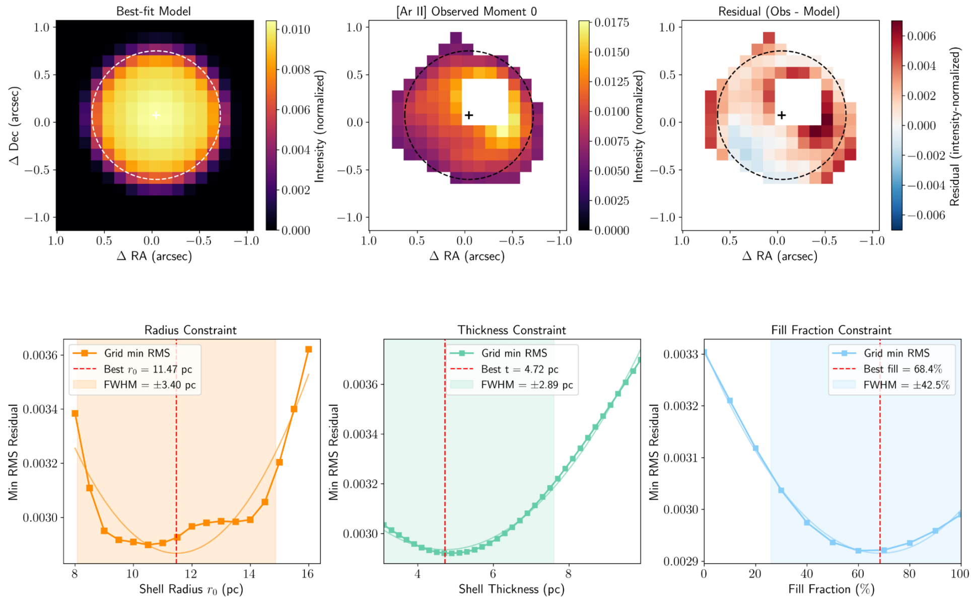
Figure 5. from Kaitlyn E. Sheriff et al 2026 Astron. J. 172 doi:10.3847/1538-3881/aea6ac https://dx.doi.org/10.3847/1538-3881/aea6ac © 2026. The Author(s). Published by the American Astronomical Society.
