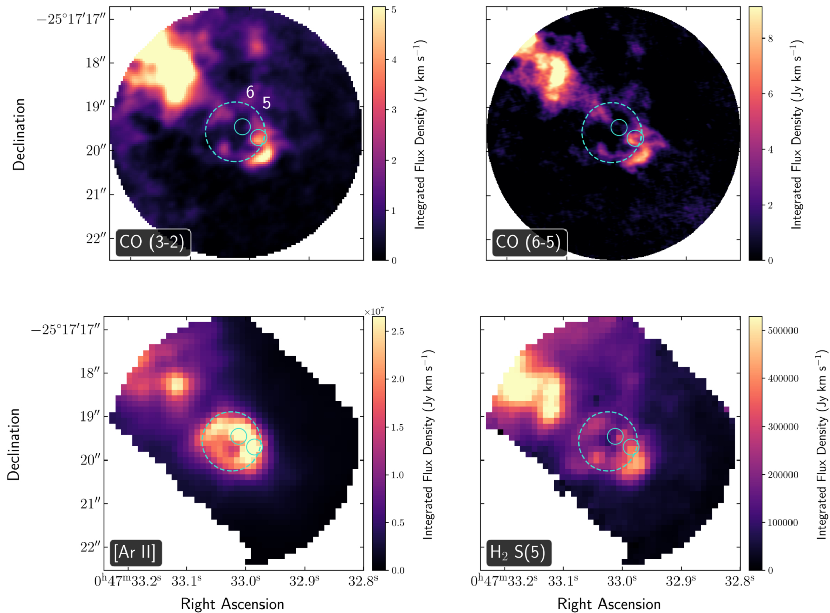
Figure 4. from Kaitlyn E. Sheriff et al 2026 Astron. J. 172 doi:10.3847/1538-3881/aea6ac https://dx.doi.org/10.3847/1538-3881/aea6ac © 2026. The Author(s). Published by the American Astronomical Society.
