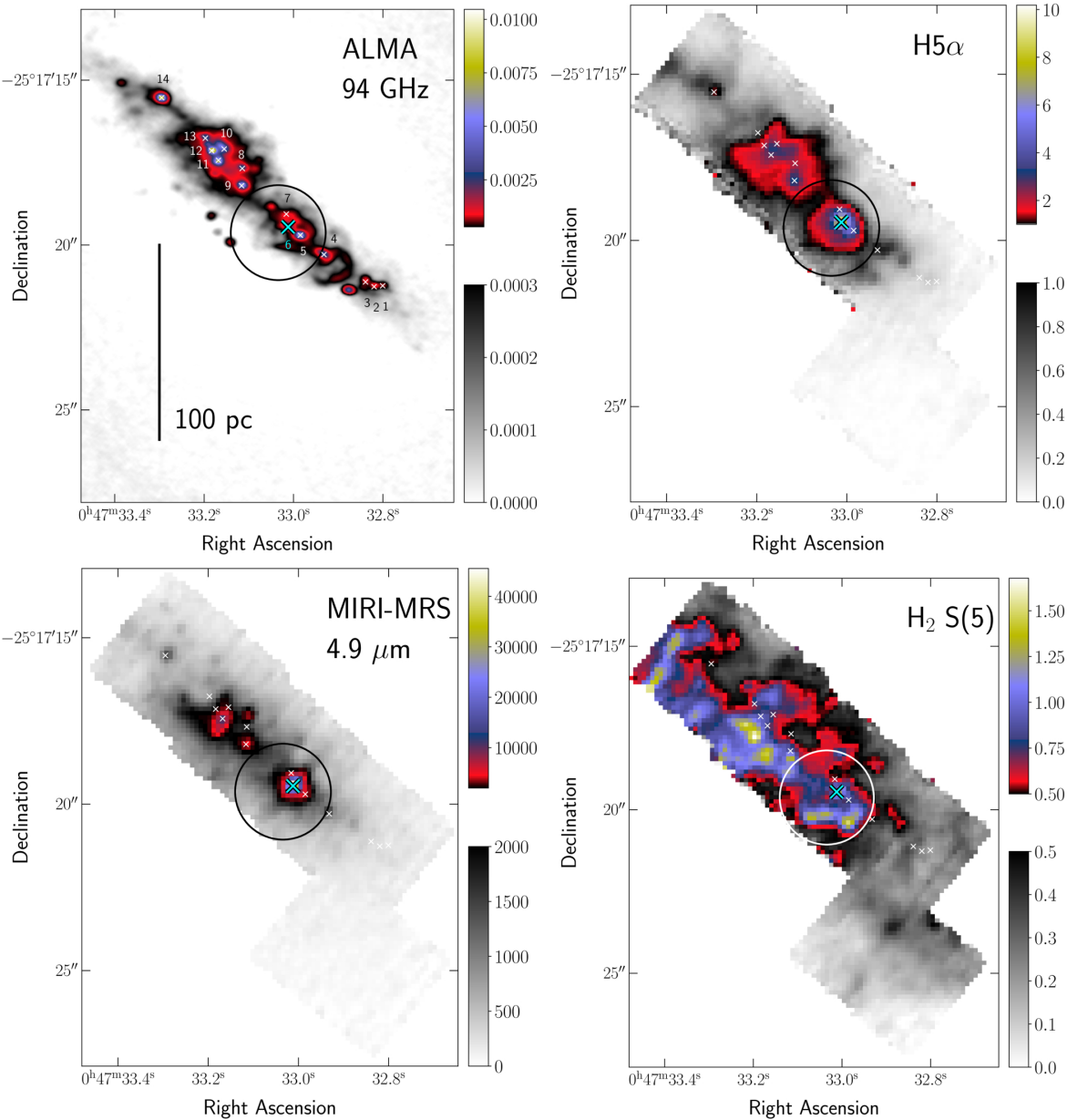
Figure 2. from Kaitlyn E. Sheriff et al 2026 Astron. J. 172 doi:10.3847/1538-3881/aea6ac https://dx.doi.org/10.3847/1538-3881/aea6ac © 2026. The Author(s). Published by the American Astronomical Society.
