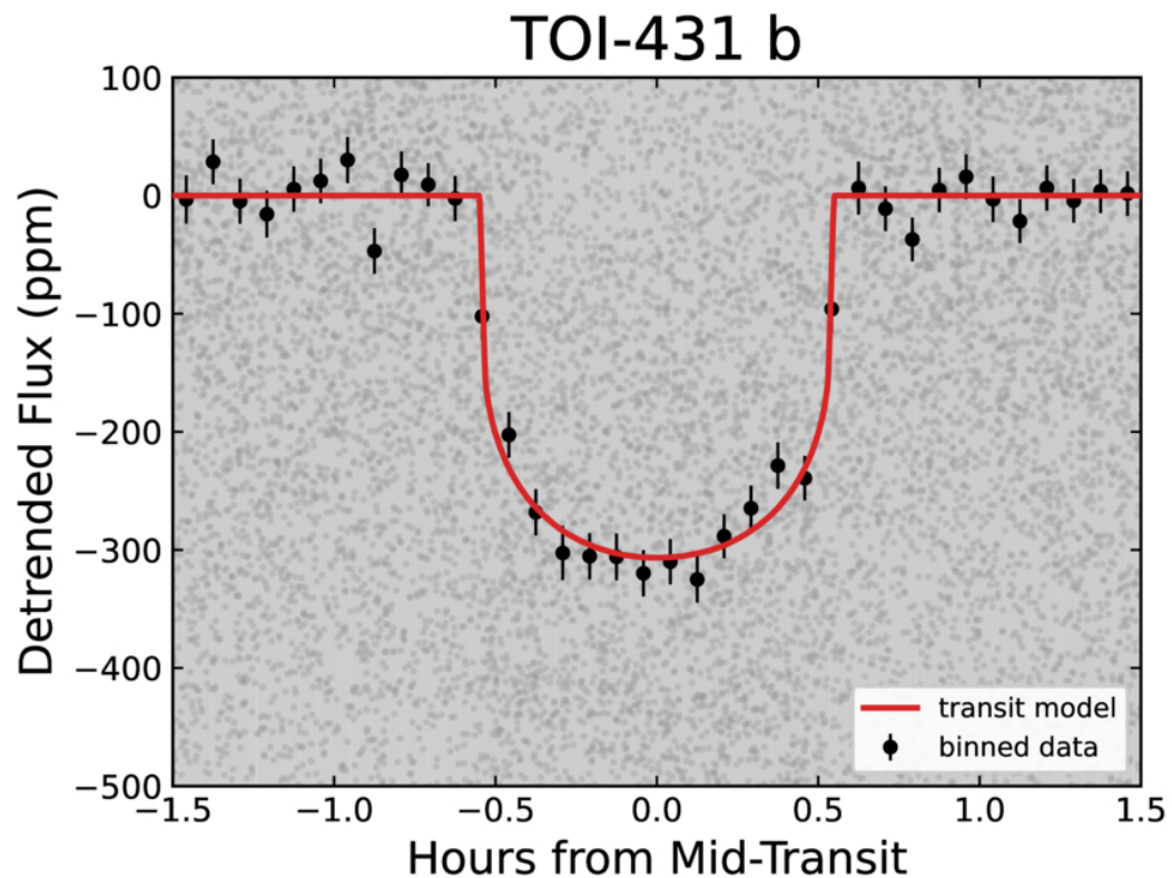
Figure A1. from Cole Smith et al 2026 Astron. J. 172 doi:10.3847/1538-3881/aea574 https://dx.doi.org/10.3847/1538-3881/aea574 © 2026. The Author(s). Published by the American Astronomical Society.
