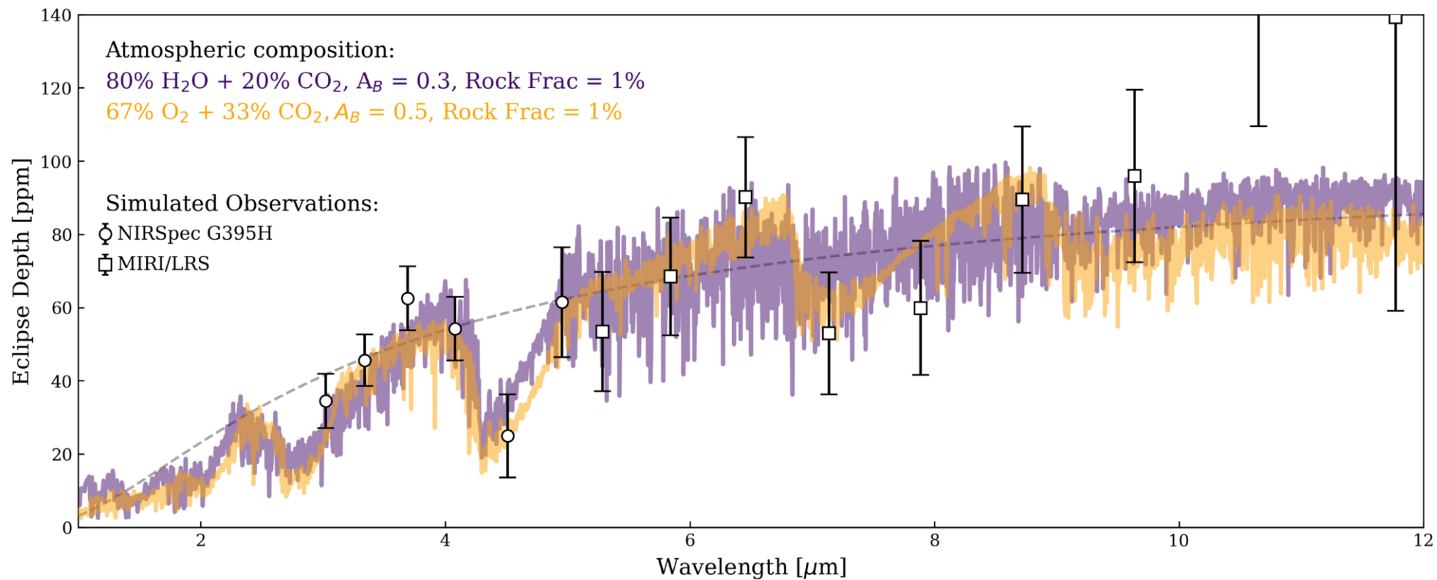
Figure 5. from Cole Smith et al 2026 Astron. J. 172 doi:10.3847/1538-3881/aea574 https://dx.doi.org/10.3847/1538-3881/aea574 © 2026. The Author(s). Published by the American Astronomical Society.
