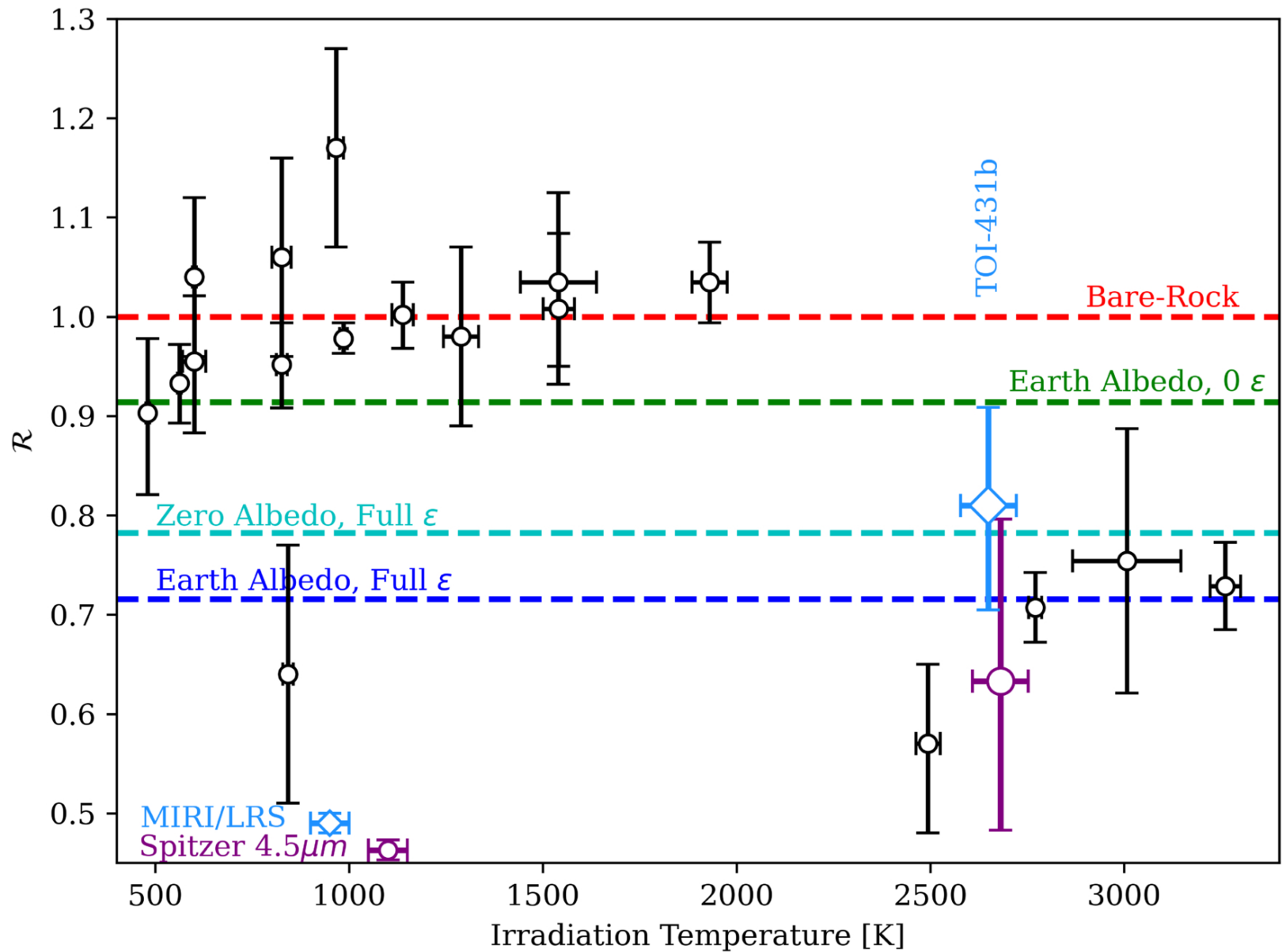
Figure 4. from Cole Smith et al 2026 Astron. J. 172 doi:10.3847/1538-3881/aea574 https://dx.doi.org/10.3847/1538-3881/aea574 © 2026. The Author(s). Published by the American Astronomical Society.
