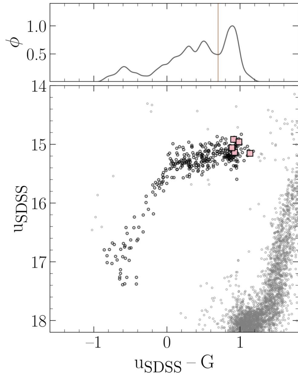
Figure 9. from Emanuele Dondoglio et al 2026 Astron. J. 172 doi:10.3847/1538-3881/aea564 https://dx.doi.org/10.3847/1538-3881/aea564 © 2026. The Author(s). Published by the American Astronomical Society.
