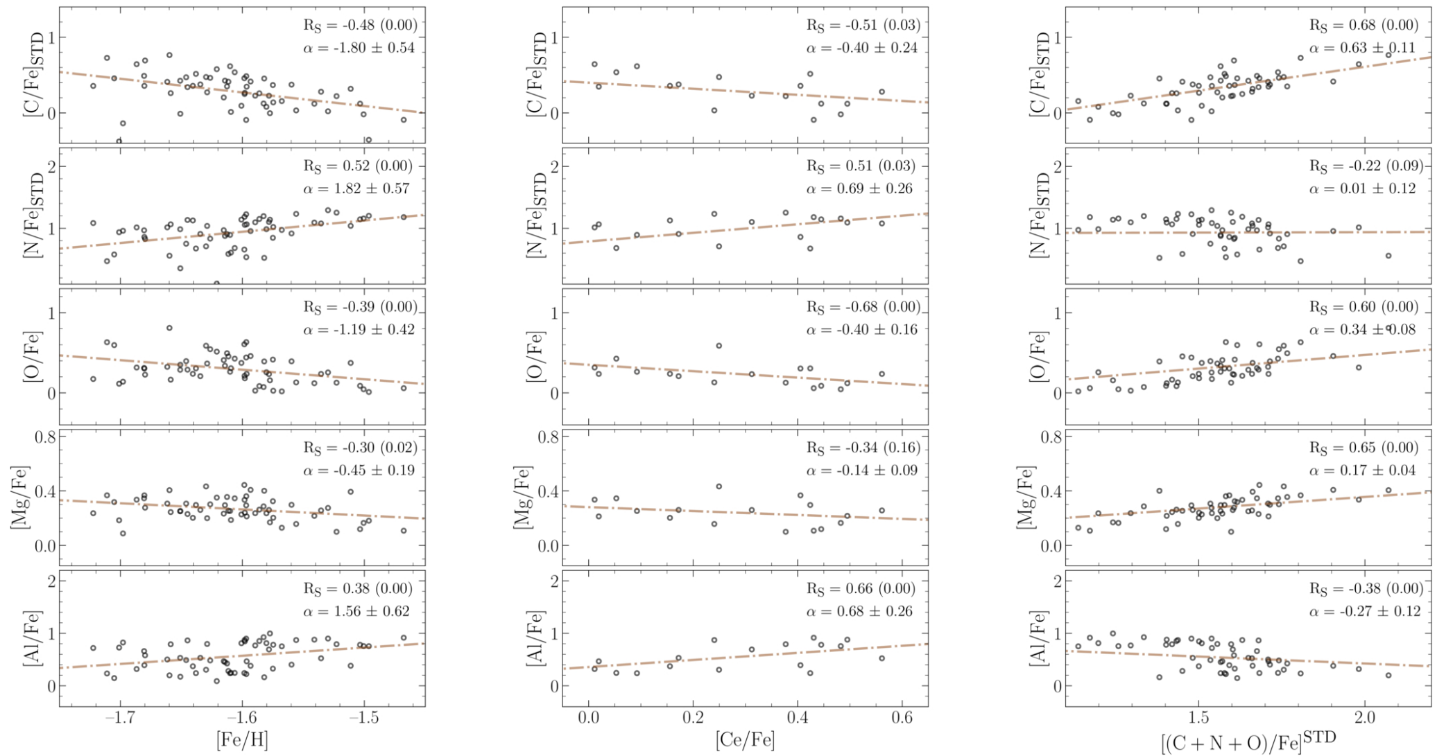
Figure 8. from Emanuele Dondoglio et al 2026 Astron. J. 172 doi:10.3847/1538-3881/aea564 https://dx.doi.org/10.3847/1538-3881/aea564 © 2026. The Author(s). Published by the American Astronomical Society.
