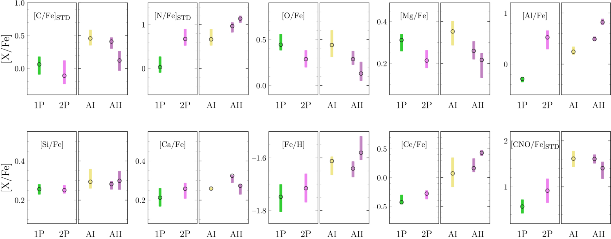
Figure 7. from Emanuele Dondoglio et al 2026 Astron. J. 172 doi:10.3847/1538-3881/aea564 https://dx.doi.org/10.3847/1538-3881/aea564 © 2026. The Author(s). Published by the American Astronomical Society.
