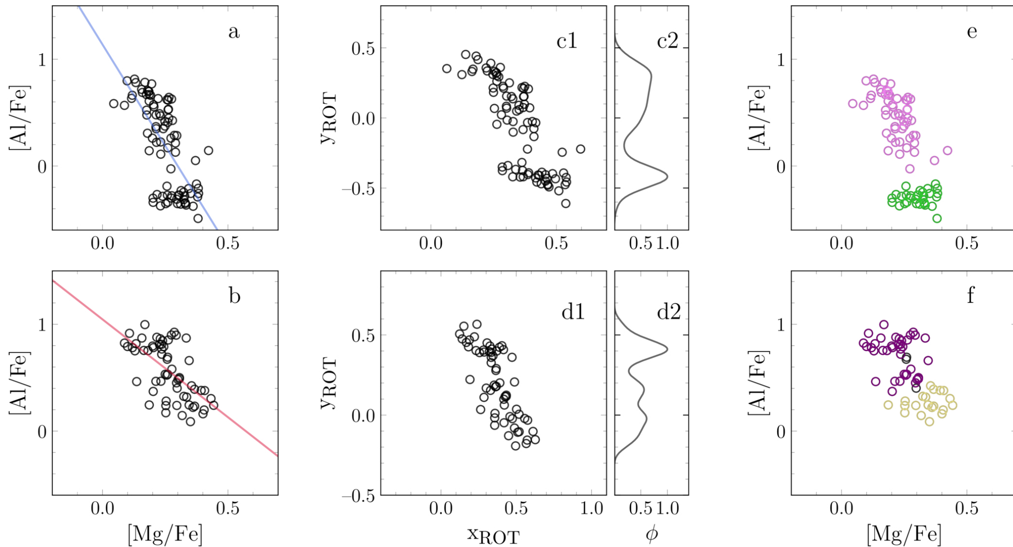
Figure 5. from Emanuele Dondoglio et al 2026 Astron. J. 172 doi:10.3847/1538-3881/aea564 https://dx.doi.org/10.3847/1538-3881/aea564 © 2026. The Author(s). Published by the American Astronomical Society.
