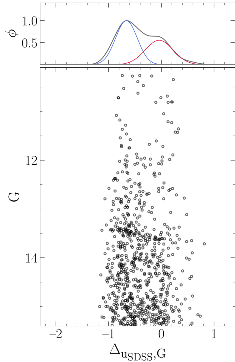
Figure 4. from Emanuele Dondoglio et al 2026 Astron. J. 172 doi:10.3847/1538-3881/aea564 https://dx.doi.org/10.3847/1538-3881/aea564 © 2026. The Author(s). Published by the American Astronomical Society.
