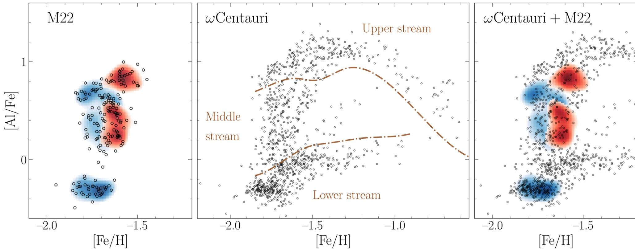
Figure 11. from Emanuele Dondoglio et al 2026 Astron. J. 172 doi:10.3847/1538-3881/aea564 https://dx.doi.org/10.3847/1538-3881/aea564 © 2026. The Author(s). Published by the American Astronomical Society.
