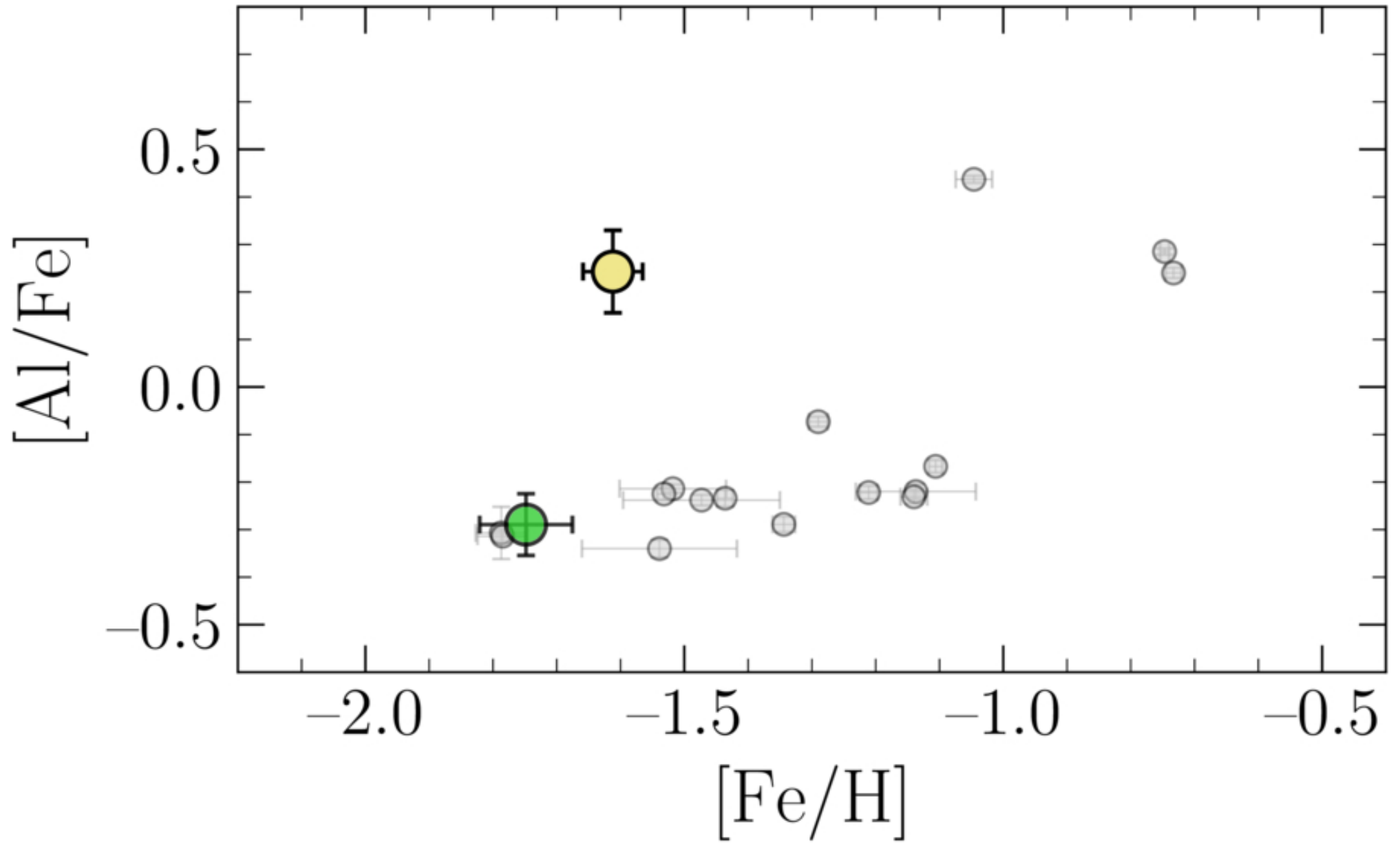
Figure 10. from Emanuele Dondoglio et al 2026 Astron. J. 172 doi:10.3847/1538-3881/aea564 https://dx.doi.org/10.3847/1538-3881/aea564 © 2026. The Author(s). Published by the American Astronomical Society.
