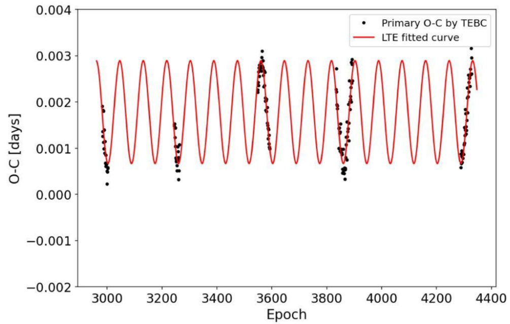
Figure 8. from Supattra Wongsriya et al 2026 Astron. J. 172 doi:10.3847/1538-3881/aea3f1 https://dx.doi.org/10.3847/1538-3881/aea3f1 © 2026. The Author(s). Published by the American Astronomical Society.
