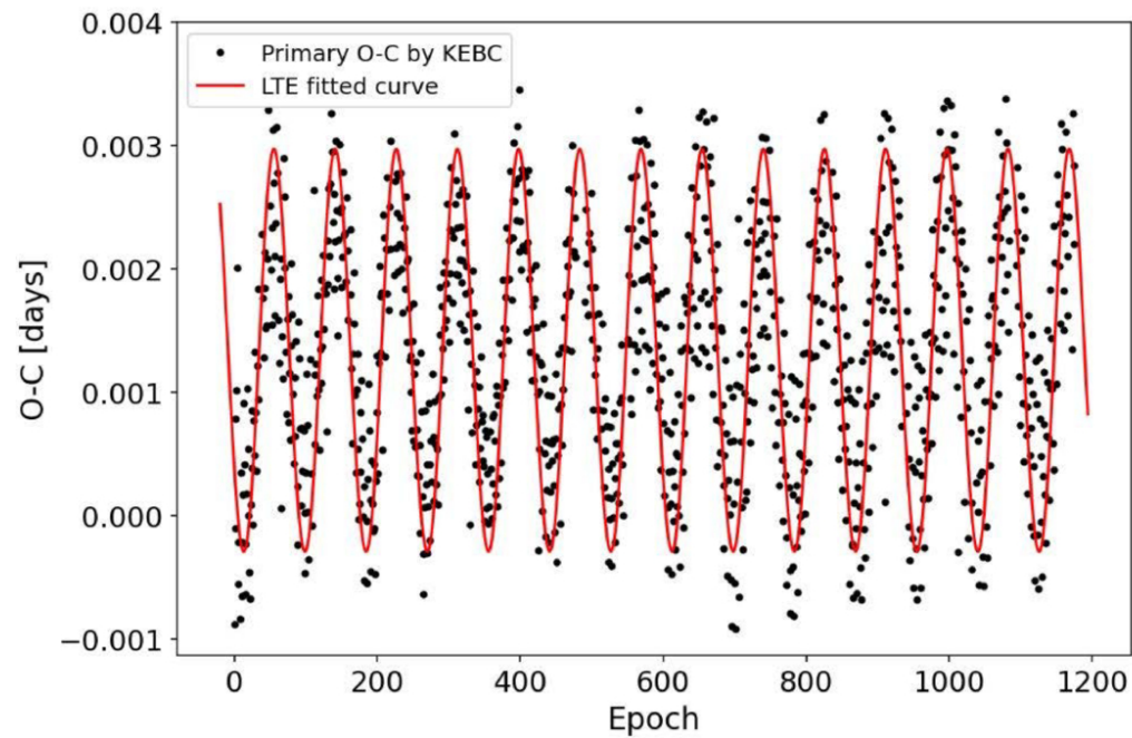
Figure 7. from Supattra Wongsriya et al 2026 Astron. J. 172 doi:10.3847/1538-3881/aea3f1 https://dx.doi.org/10.3847/1538-3881/aea3f1 © 2026. The Author(s). Published by the American Astronomical Society.
