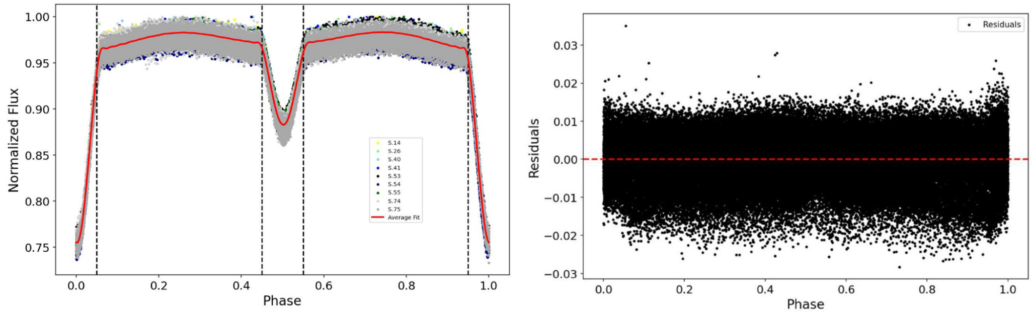
Figure 4. from Supattra Wongsriya et al 2026 Astron. J. 172 doi:10.3847/1538-3881/aea3f1 https://dx.doi.org/10.3847/1538-3881/aea3f1 © 2026. The Author(s). Published by the American Astronomical Society.
