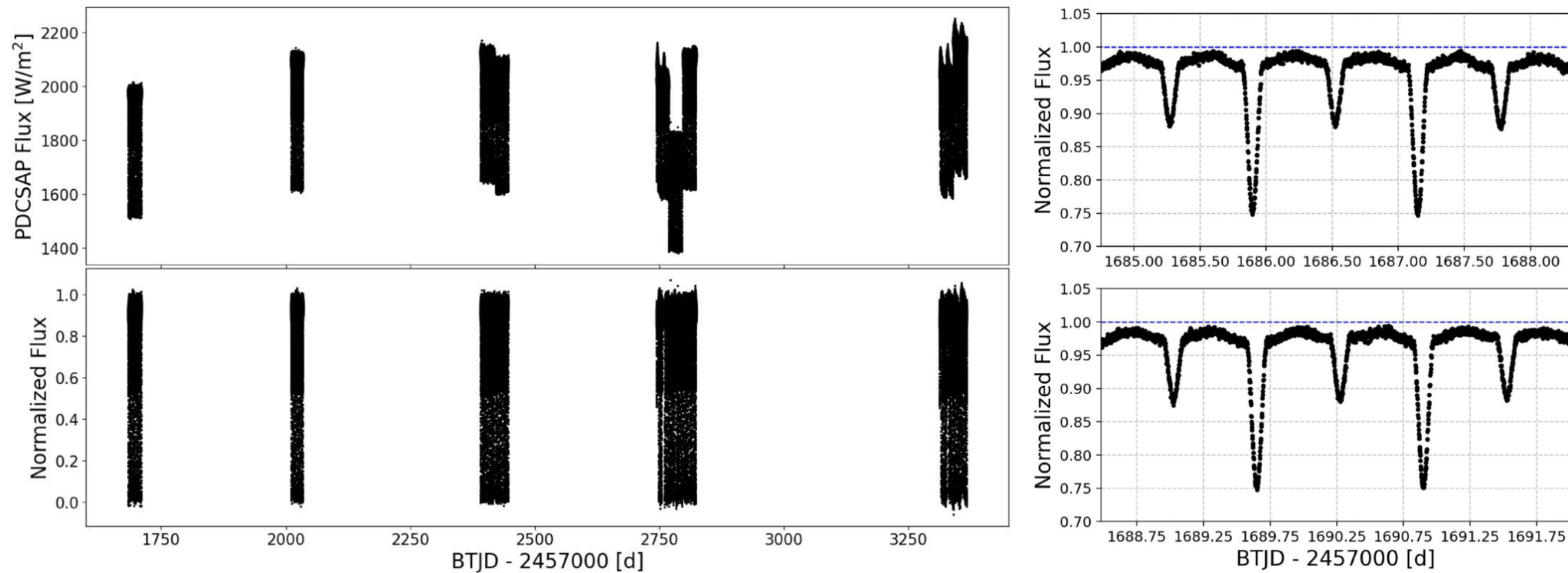
Figure 3. from Supattra Wongsriya et al 2026 Astron. J. 172 doi:10.3847/1538-3881/aea3f1 https://dx.doi.org/10.3847/1538-3881/aea3f1 © 2026. The Author(s). Published by the American Astronomical Society.
