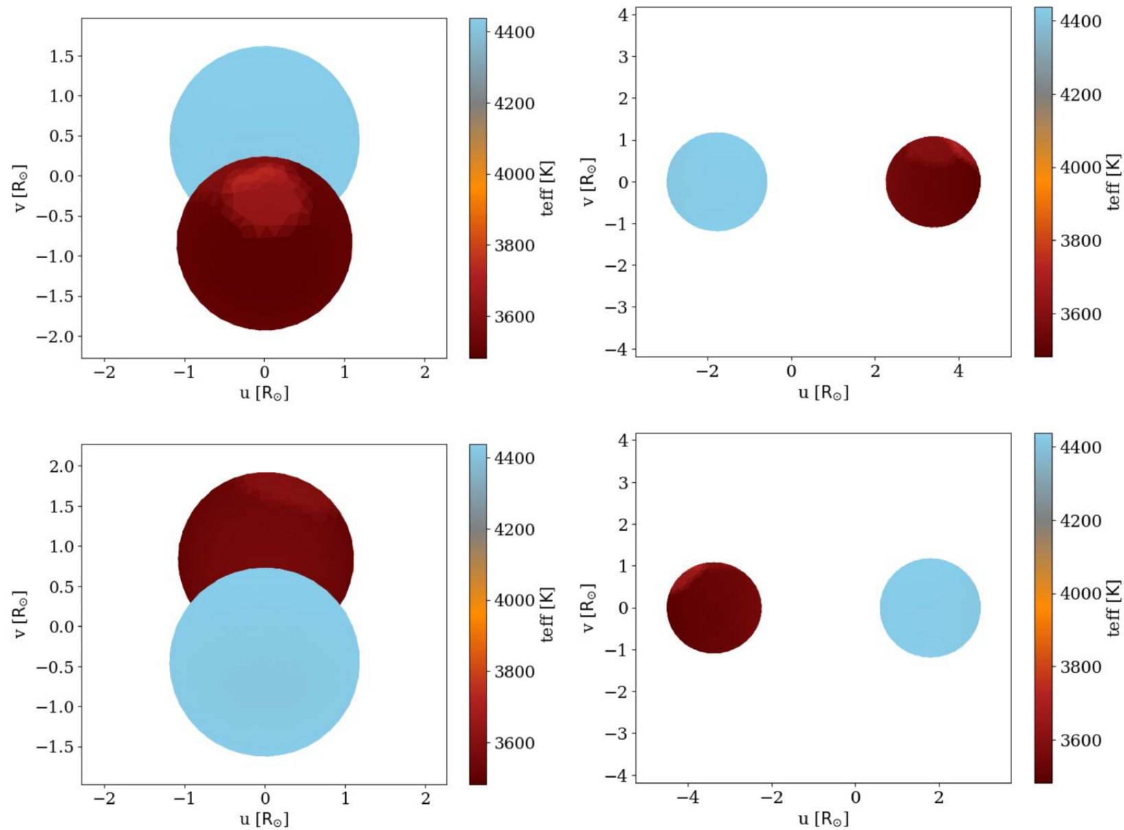
Figure 16. from Supattra Wongsriya et al 2026 Astron. J. 172 doi:10.3847/1538-3881/aea3f1 https://dx.doi.org/10.3847/1538-3881/aea3f1 © 2026. The Author(s). Published by the American Astronomical Society.
