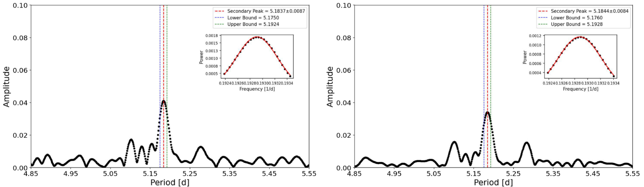
Figure 12. from Supattra Wongsriya et al 2026 Astron. J. 172 doi:10.3847/1538-3881/aea3f1 https://dx.doi.org/10.3847/1538-3881/aea3f1 © 2026. The Author(s). Published by the American Astronomical Society.
