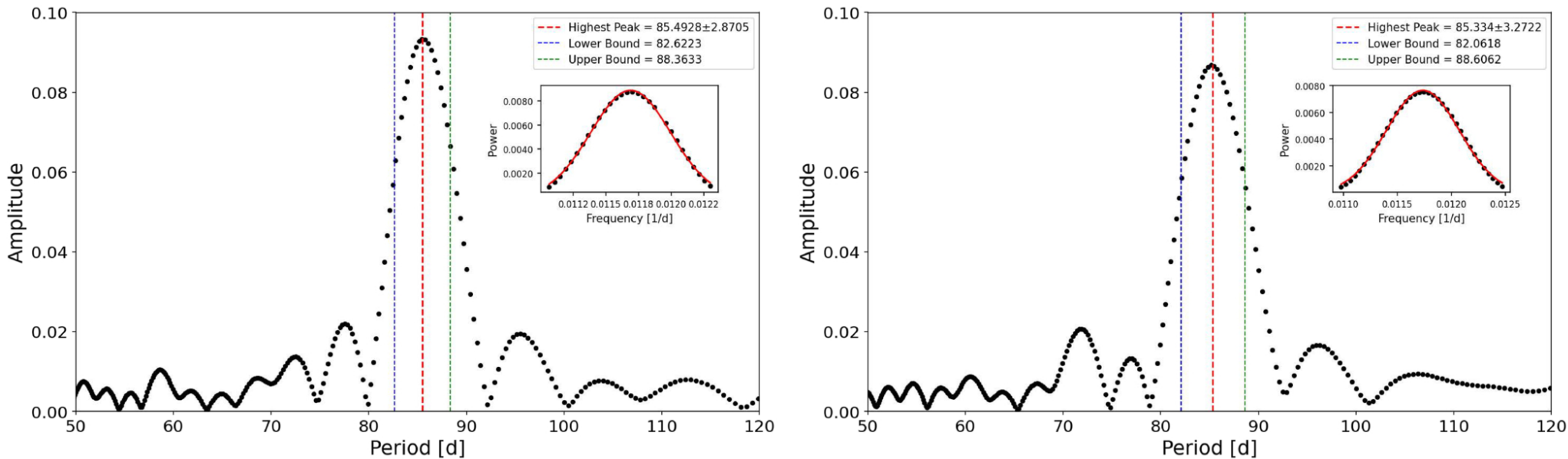
Figure 10. from Supattra Wongsriya et al 2026 Astron. J. 172 doi:10.3847/1538-3881/aea3f1 https://dx.doi.org/10.3847/1538-3881/aea3f1 © 2026. The Author(s). Published by the American Astronomical Society.
