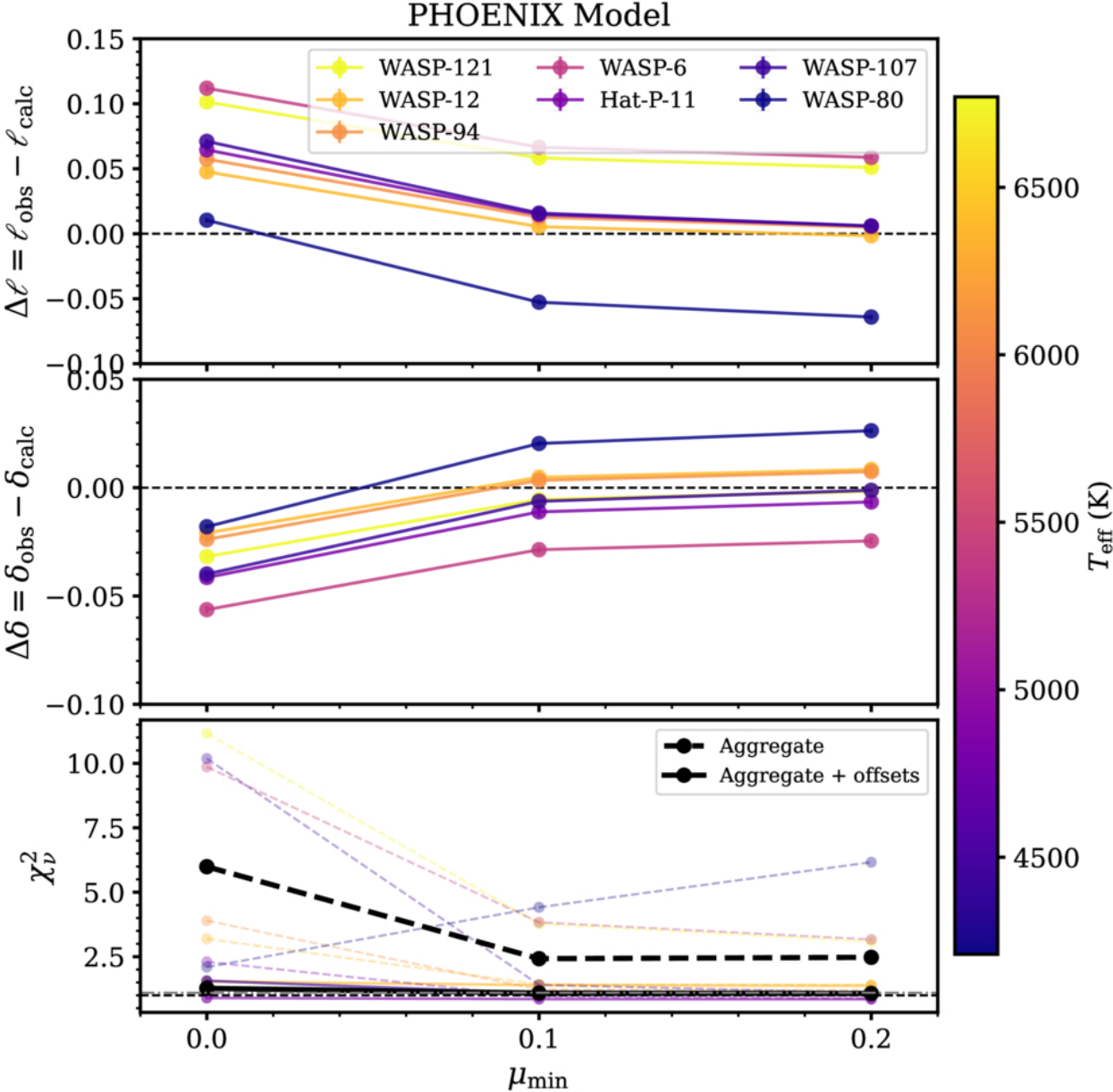
Figure 9. from David K. Sing et al 2026 Astron. J. 172 doi:10.3847/1538-3881/aea21e https://dx.doi.org/10.3847/1538-3881/aea21e © 2026. The Author(s). Published by the American Astronomical Society.
