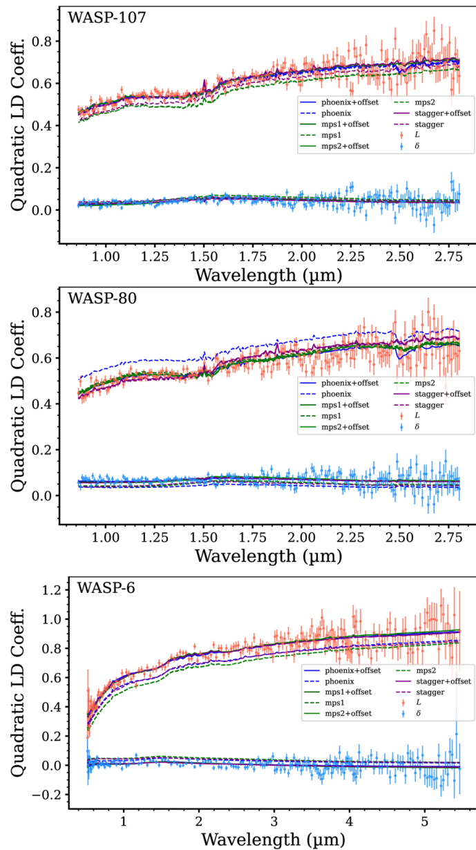
Figure 7. from David K. Sing et al 2026 Astron. J. 172 doi:10.3847/1538-3881/aea21e https://dx.doi.org/10.3847/1538-3881/aea21e © 2026. The Author(s). Published by the American Astronomical Society.
