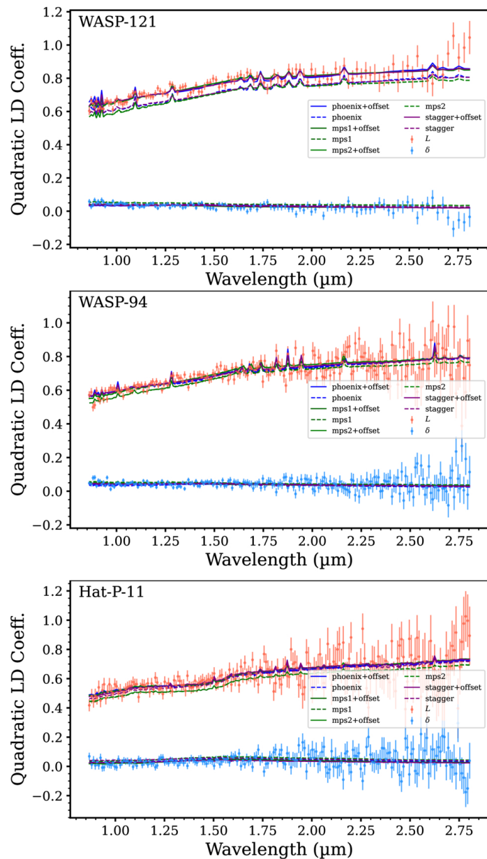
Figure 6. from David K. Sing et al 2026 Astron. J. 172 doi:10.3847/1538-3881/aea21e https://dx.doi.org/10.3847/1538-3881/aea21e © 2026. The Author(s). Published by the American Astronomical Society.
