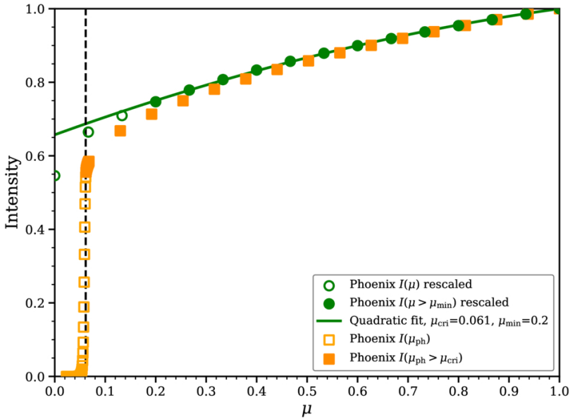
Figure 4. from David K. Sing et al 2026 Astron. J. 172 doi:10.3847/1538-3881/aea21e https://dx.doi.org/10.3847/1538-3881/aea21e © 2026. The Author(s). Published by the American Astronomical Society.
