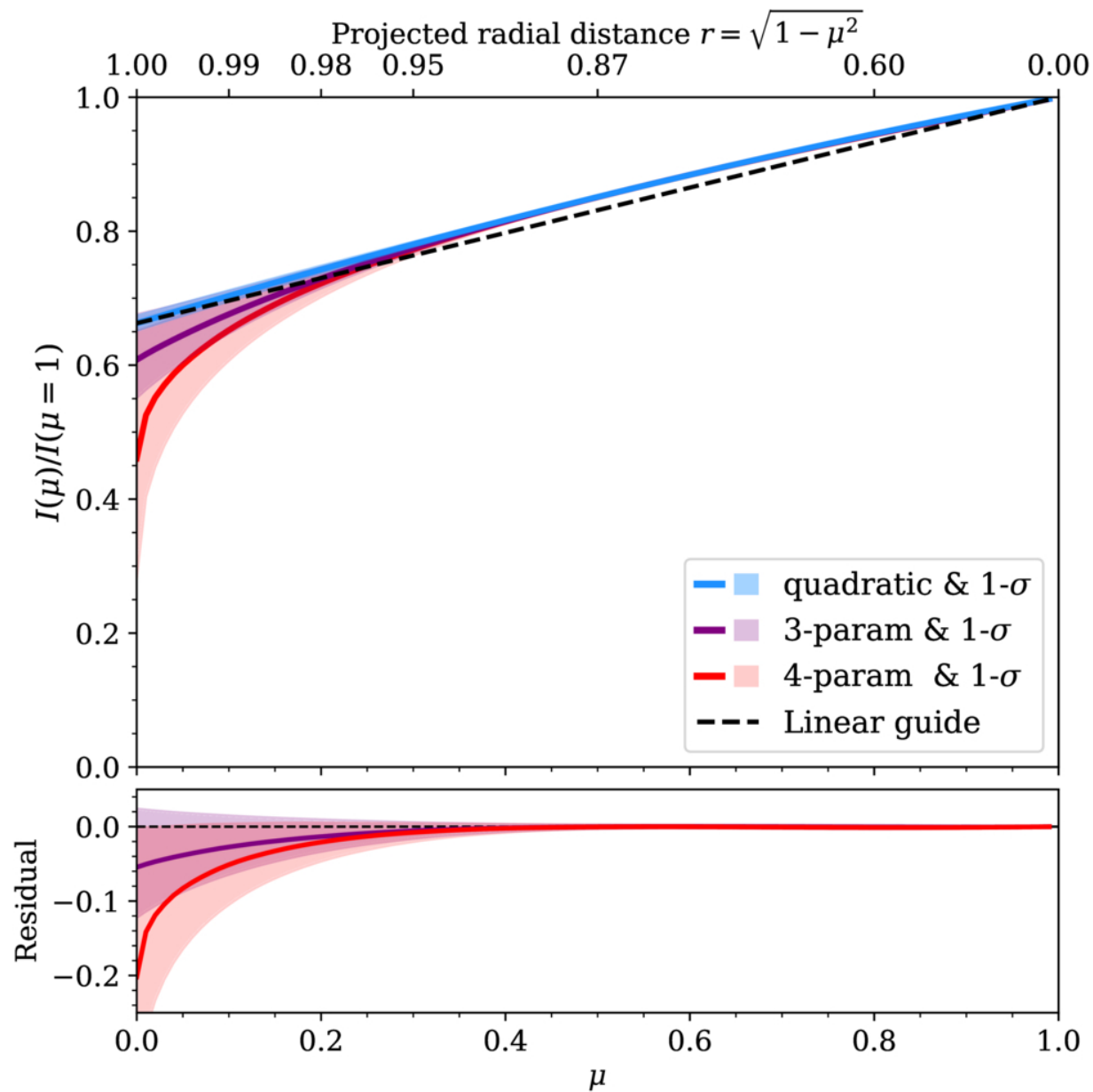
Figure 2. from David K. Sing et al 2026 Astron. J. 172 doi:10.3847/1538-3881/aea21e https://dx.doi.org/10.3847/1538-3881/aea21e © 2026. The Author(s). Published by the American Astronomical Society.
