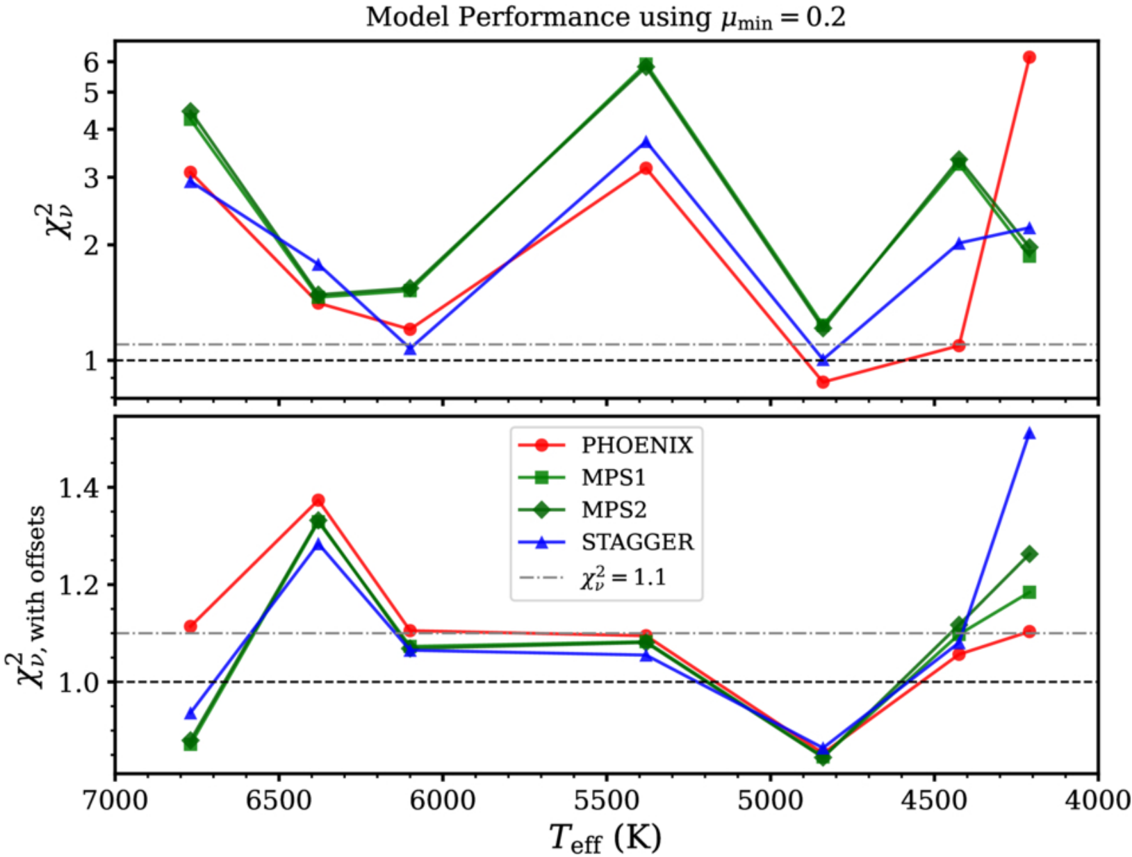
Figure 12. from David K. Sing et al 2026 Astron. J. 172 doi:10.3847/1538-3881/aea21e https://dx.doi.org/10.3847/1538-3881/aea21e © 2026. The Author(s). Published by the American Astronomical Society.
