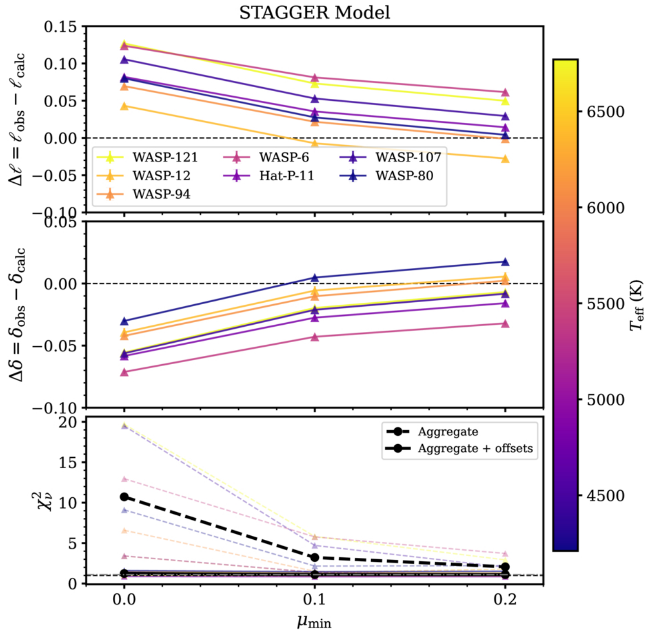
Figure 11. from David K. Sing et al 2026 Astron. J. 172 doi:10.3847/1538-3881/aea21e https://dx.doi.org/10.3847/1538-3881/aea21e © 2026. The Author(s). Published by the American Astronomical Society.
