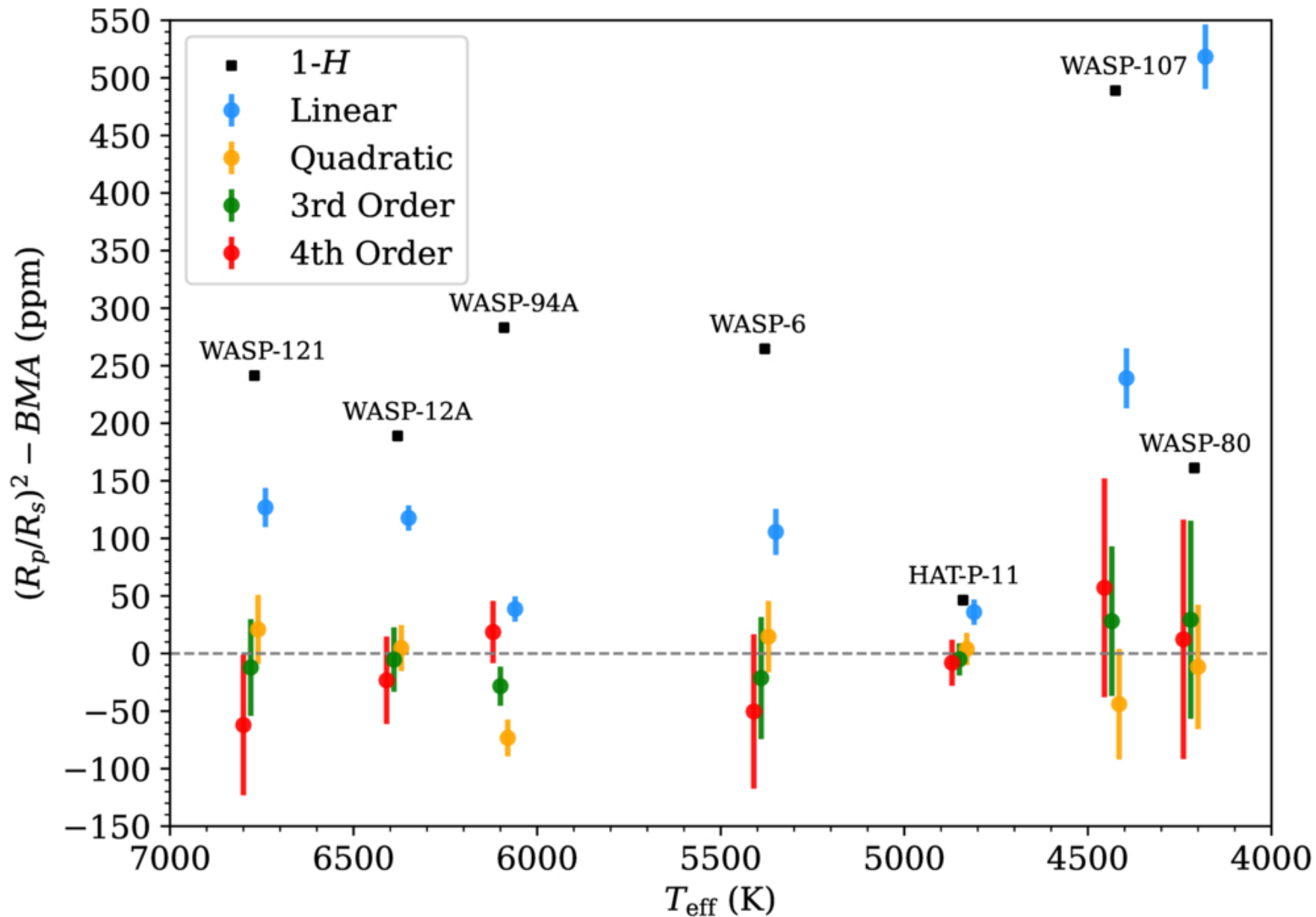
Figure 1. from David K. Sing et al 2026 Astron. J. 172 doi:10.3847/1538-3881/aea21e https://dx.doi.org/10.3847/1538-3881/aea21e © 2026. The Author(s). Published by the American Astronomical Society.
