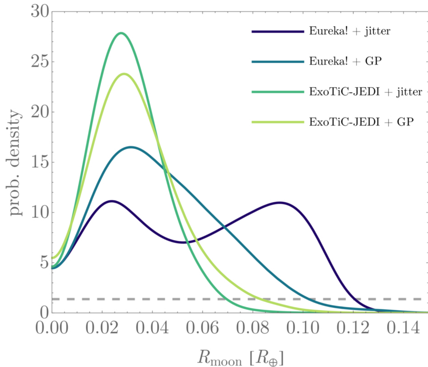
Figure 6. from David Kipping 2026 Astron. J. 172 doi:10.3847/1538-3881/aea21d https://dx.doi.org/10.3847/1538-3881/aea21d © 2026. The Author(s). Published by the American Astronomical Society.
