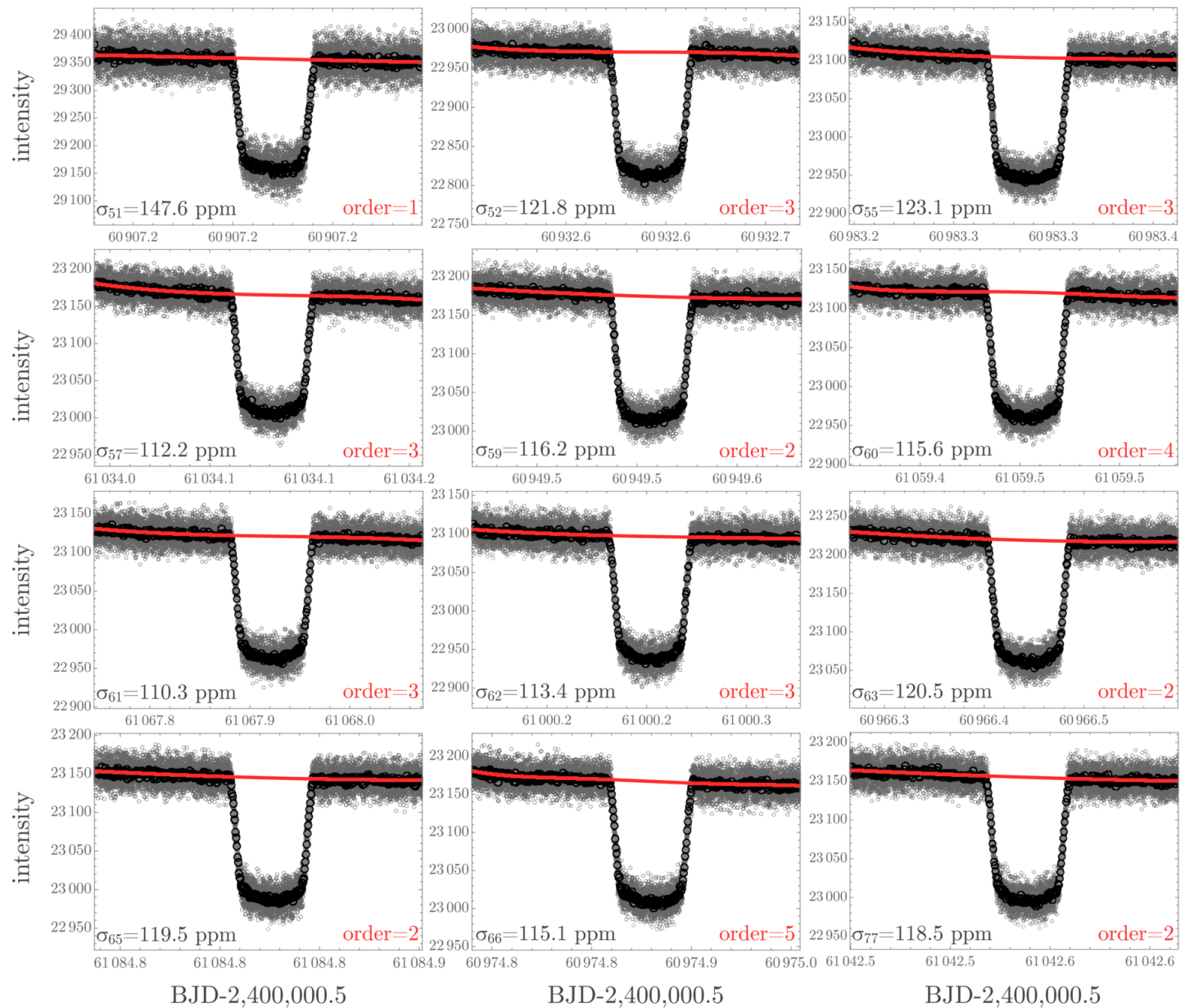
Figure 2. from David Kipping 2026 Astron. J. 172 doi:10.3847/1538-3881/aea21d https://dx.doi.org/10.3847/1538-3881/aea21d © 2026. The Author(s). Published by the American Astronomical Society.
