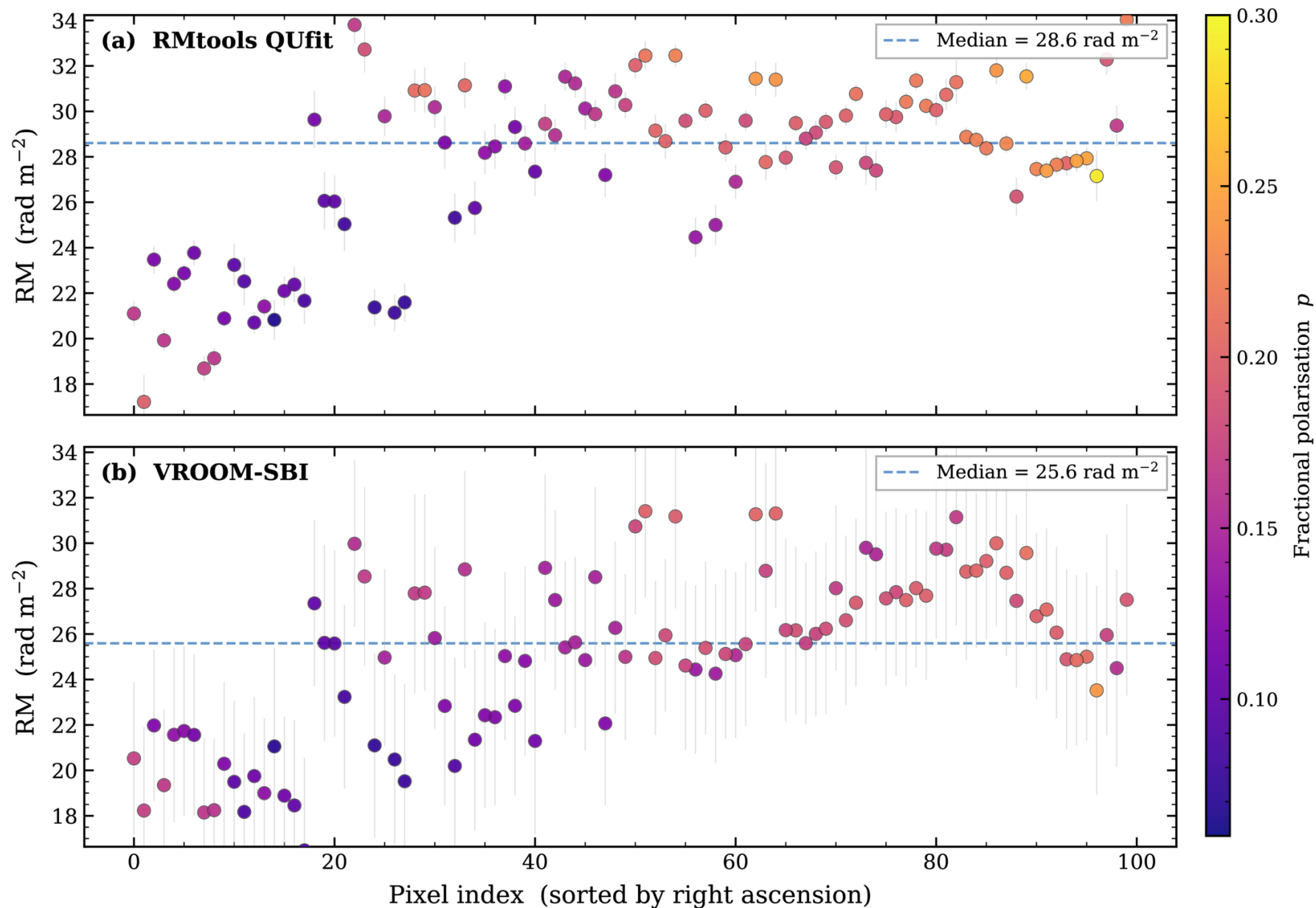
Figure 8. from Arpan Pal and Preshanth Jagannathan 2026 Astron. J. 172 doi:10.3847/1538-3881/aea208 https://dx.doi.org/10.3847/1538-3881/aea208 © 2026. The Author(s). Published by the American Astronomical Society.
