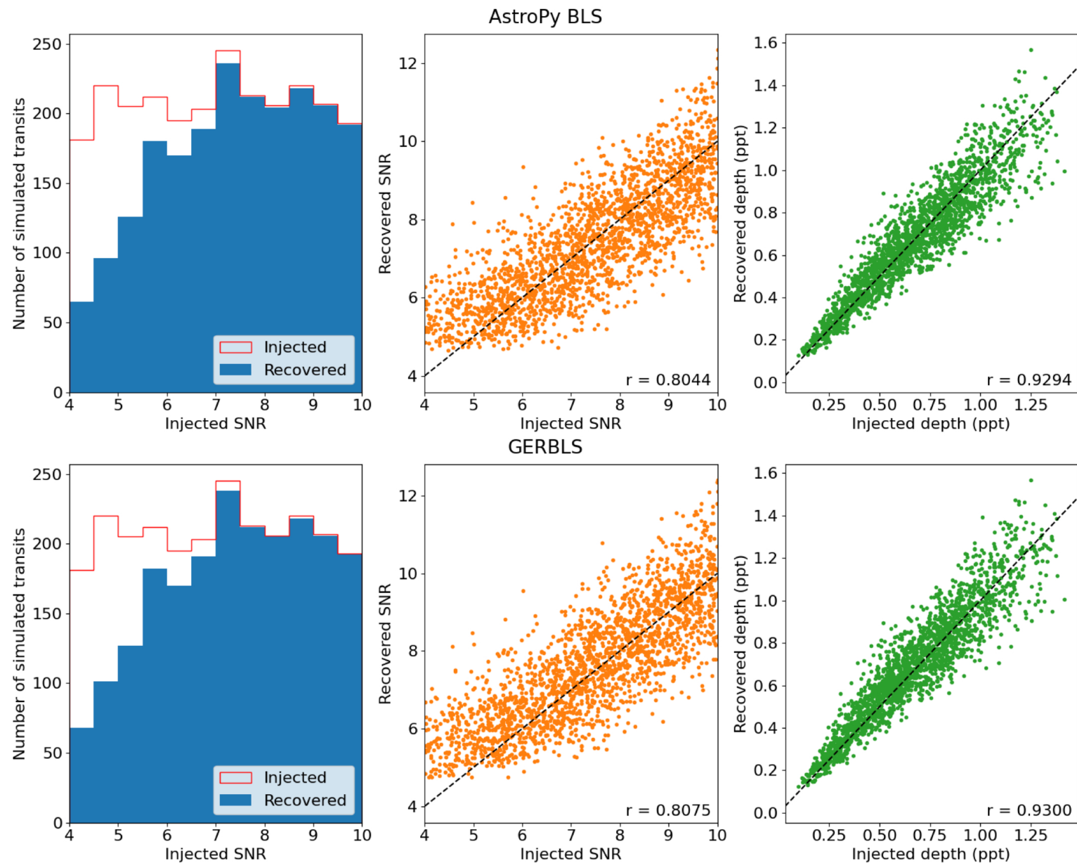
Figure 6. from Kristo Ment et al 2026 Astron. J. 172 doi:10.3847/1538-3881/aea0c8 https://dx.doi.org/10.3847/1538-3881/aea0c8 © 2026. The Author(s). Published by the American Astronomical Society.
