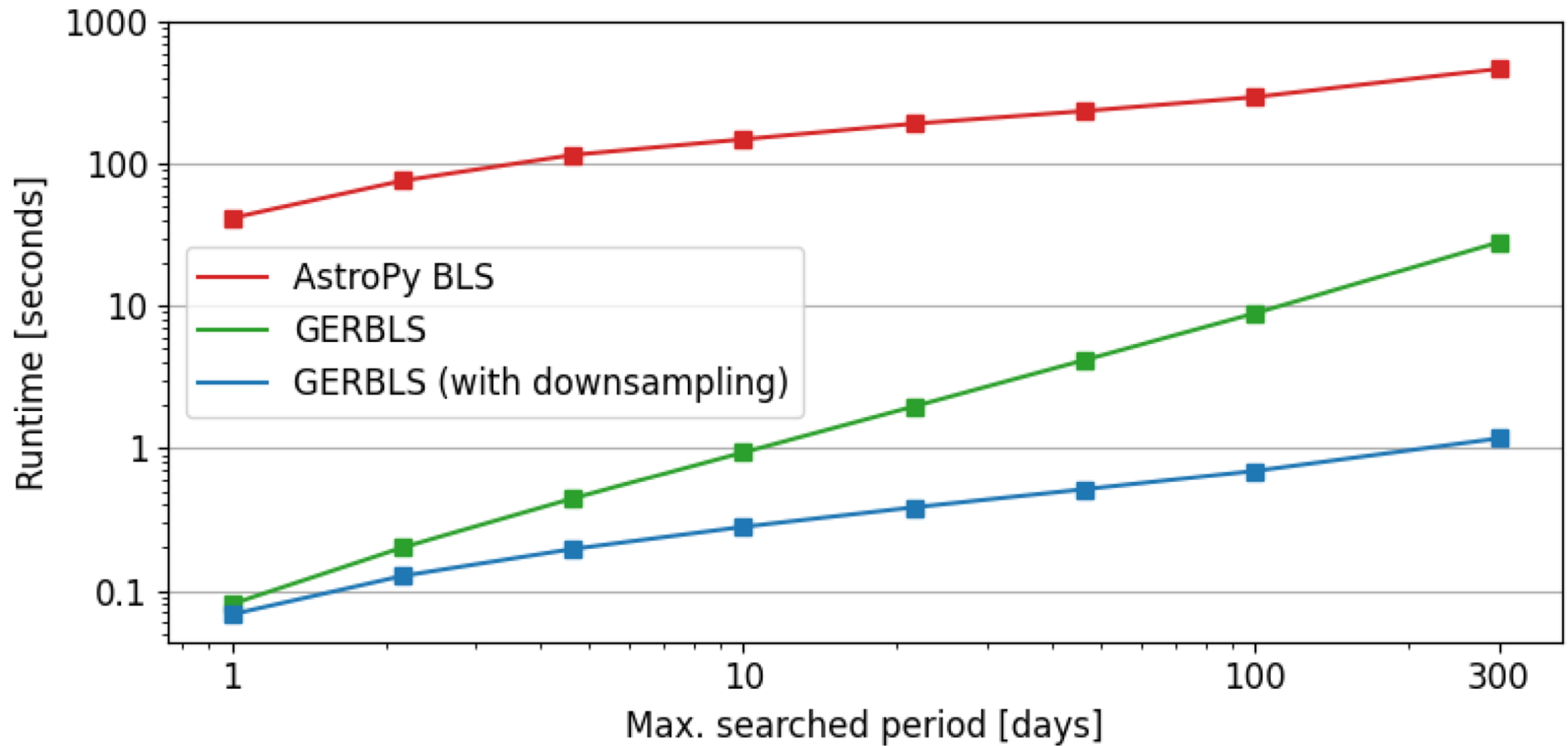
Figure 5. from Kristo Ment et al 2026 Astron. J. 172 doi:10.3847/1538-3881/aea0c8 https://dx.doi.org/10.3847/1538-3881/aea0c8 © 2026. The Author(s). Published by the American Astronomical Society.
