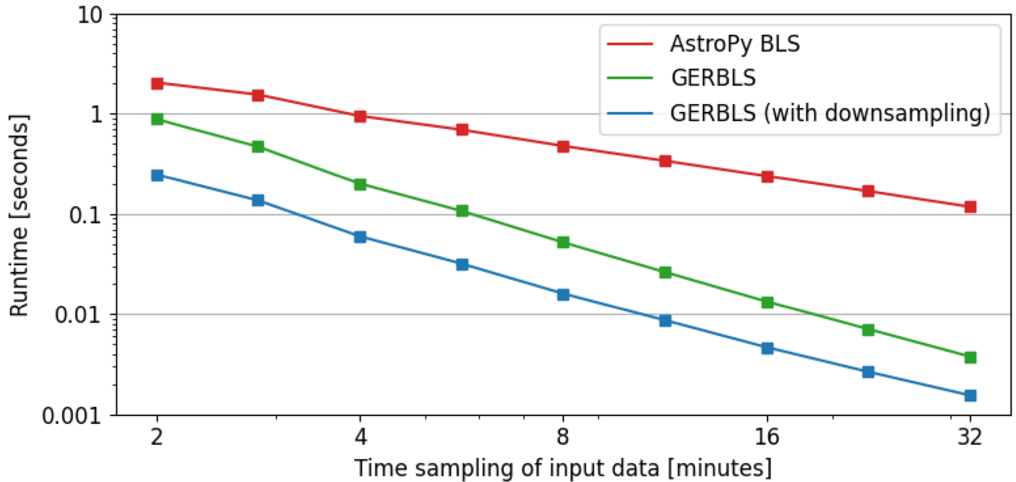
Figure 4. from Kristo Ment et al 2026 Astron. J. 172 doi:10.3847/1538-3881/aea0c8 https://dx.doi.org/10.3847/1538-3881/aea0c8 © 2026. The Author(s). Published by the American Astronomical Society.
