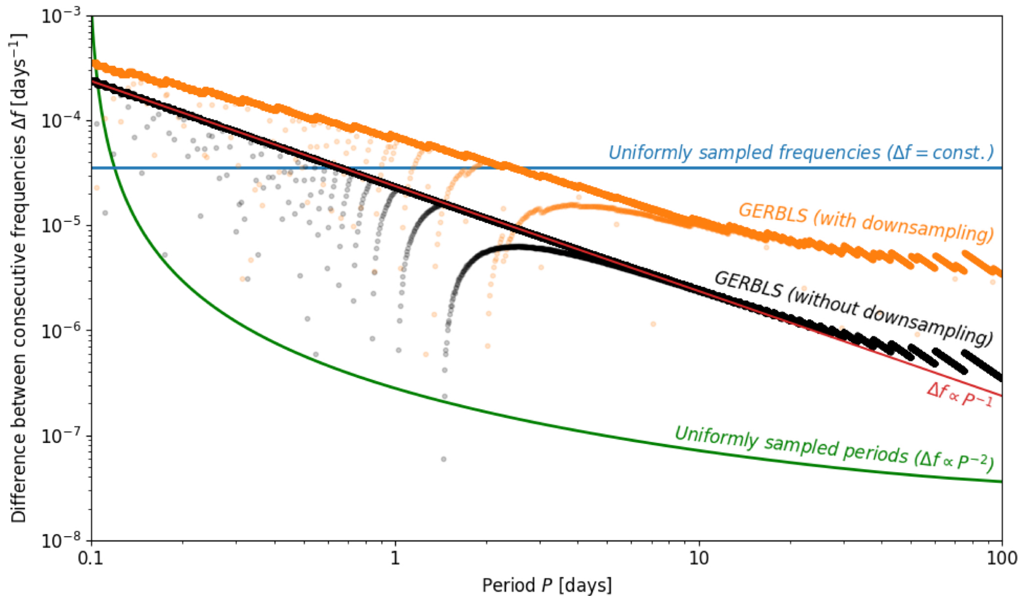
Figure 2. from Kristo Ment et al 2026 Astron. J. 172 doi:10.3847/1538-3881/aea0c8 https://dx.doi.org/10.3847/1538-3881/aea0c8 © 2026. The Author(s). Published by the American Astronomical Society.
