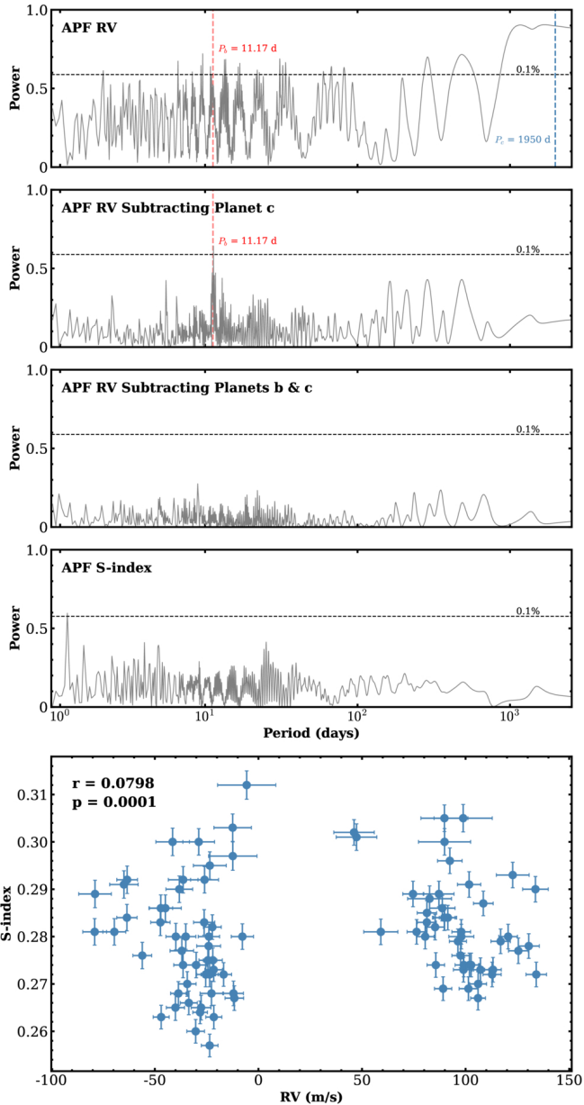
Figure 2. from Jessica A. Ranshaw et al 2026 Astron. J. 172 doi:10.3847/1538-3881/ae9ff1 https://dx.doi.org/10.3847/1538-3881/ae9ff1 © 2026. The Author(s). Published by the American Astronomical Society.
