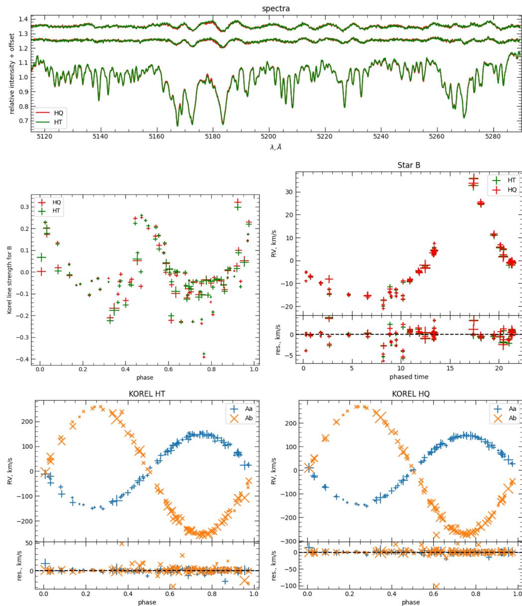
Figure 6. from Mikhail Yu. Kovalev and oa Mxa pe 2026 Astron. J. 172 doi:10.3847/1538-3881/ae9f5b https://dx.doi.org/10.3847/1538-3881/ae9f5b © 2026. The Author(s). Published by the American Astronomical Society.
