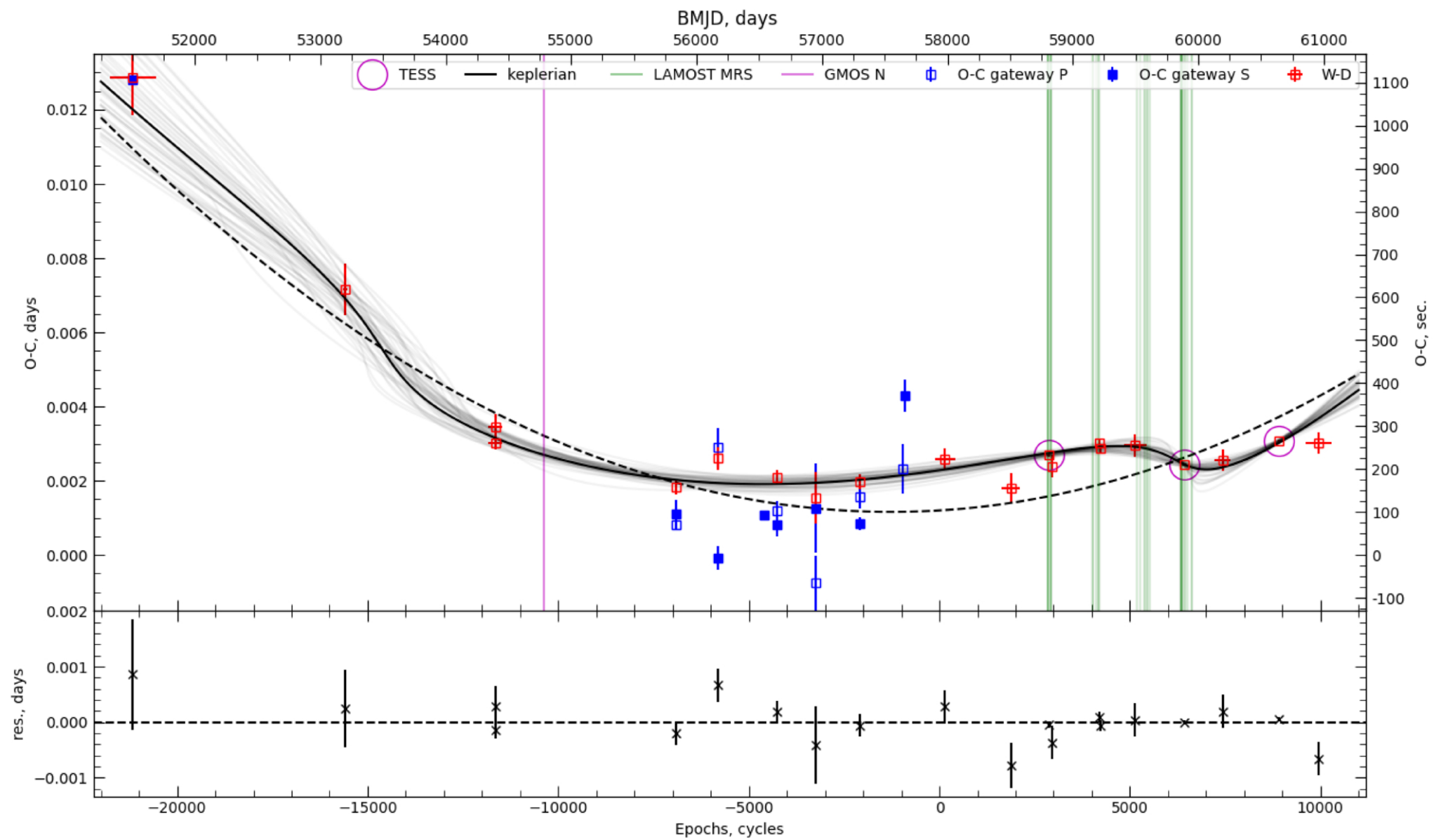
Figure 5. from Mikhail Yu. Kovalev and oa Mxa pe 2026 Astron. J. 172 doi:10.3847/1538-3881/ae9f5b https://dx.doi.org/10.3847/1538-3881/ae9f5b © 2026. The Author(s). Published by the American Astronomical Society.
