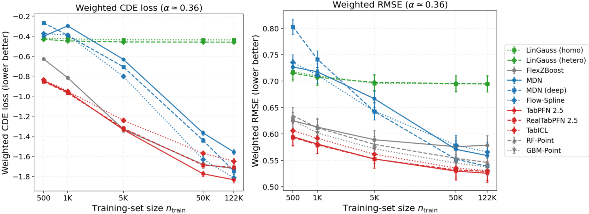
Figure 6. from Raquel R. Valena et al 2026 Astron. J. 172 doi:10.3847/1538-3881/ae9eb6 https://dx.doi.org/10.3847/1538-3881/ae9eb6 © 2026. The Author(s). Published by the American Astronomical Society.
